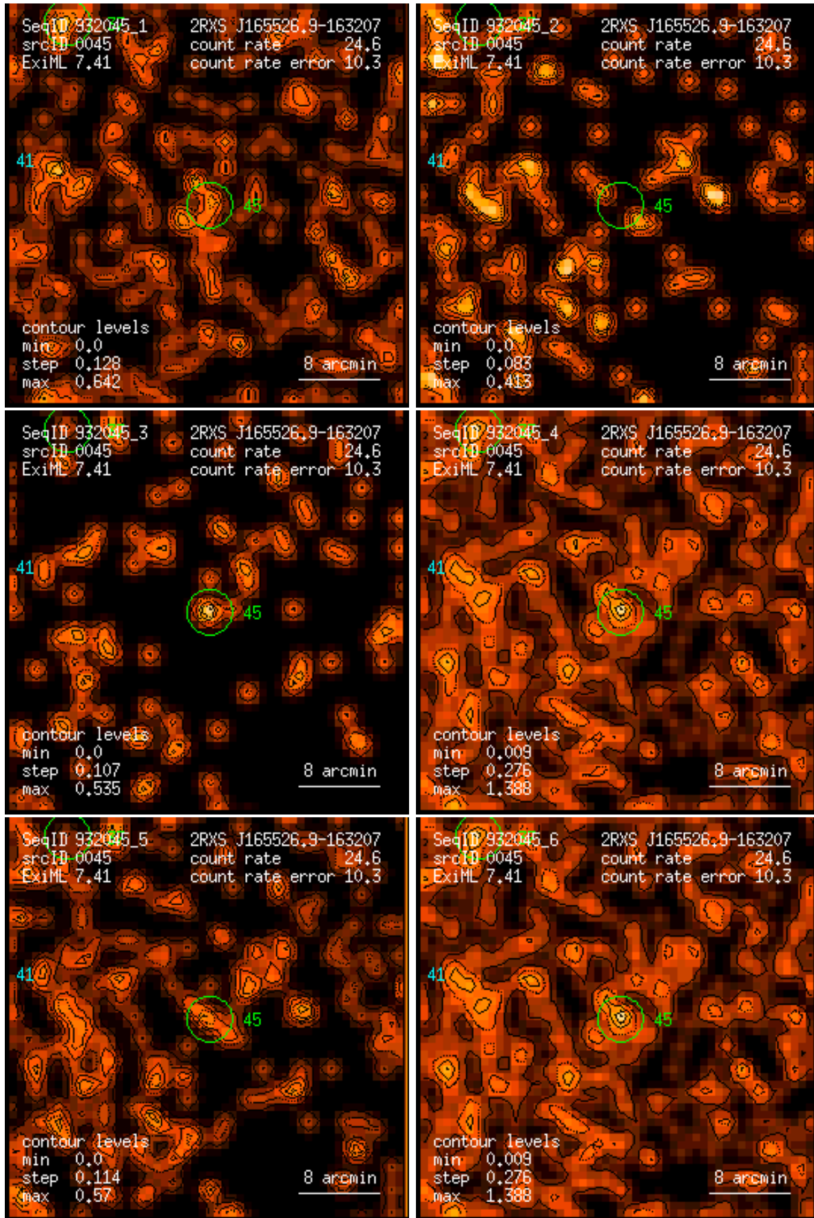
Figure 45: RASS 932045: detection 0045: band rate images, Gaussian filter: (1) PSPC channels 11 – 41, (2) 52 – 90, (3) 91 – 201, (4) 11 – 235, (5) 52 – 201, (6) 11 – 201. Broad band rates in counts/ks. Band rate contour levels in counts/ks/arcmin 2 .
