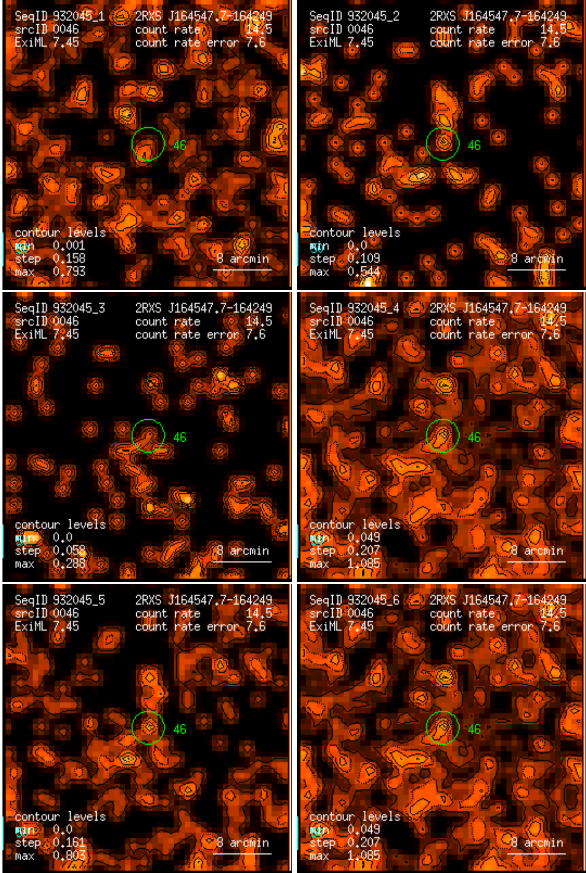
Figure 46: RASS 932045: detection 0046: band rate images, Gaussian filter: (1) PSPC channels 11 – 41, (2) 52 – 90, (3) 91 – 201, (4) 11 – 235, (5) 52 – 201, (6) 11 – 201. Broad band rates in counts/ks. Band rate contour levels in counts/ks/arcmin 2 .
