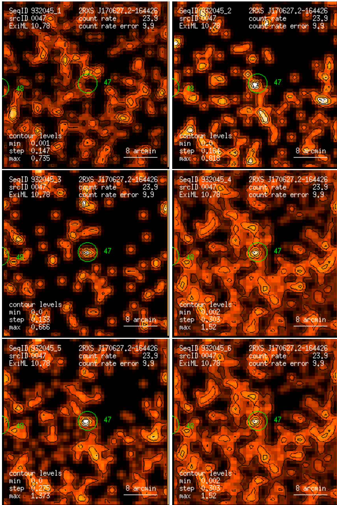
Figure 47: RASS 932045: detection 0047: band rate images, Gaussian filter: (1) PSPC channels 11 – 41, (2) 52 – 90, (3) 91 – 201, (4) 11 – 235, (5) 52 – 201, (6) 11 – 201. Broad band rates in counts/ks. Band rate contour levels in counts/ks/arcmin 2 .
