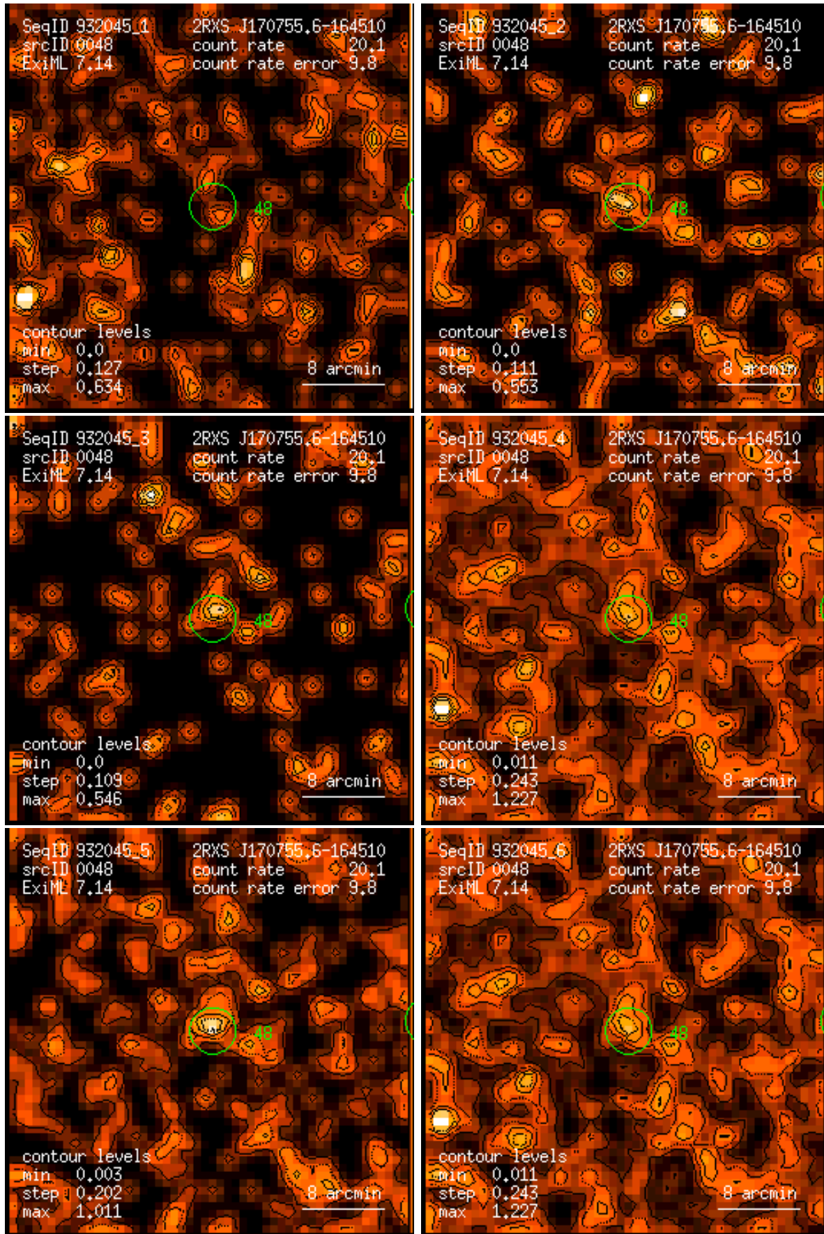
Figure 48: RASS 932045: detection 0048: band rate images, Gaussian filter: (1) PSPC channels 11 – 41, (2) 52 – 90, (3) 91 – 201, (4) 11 – 235, (5) 52 – 201, (6) 11 – 201. Broad band rates in counts/ks. Band rate contour levels in counts/ks/arcmin 2 .
