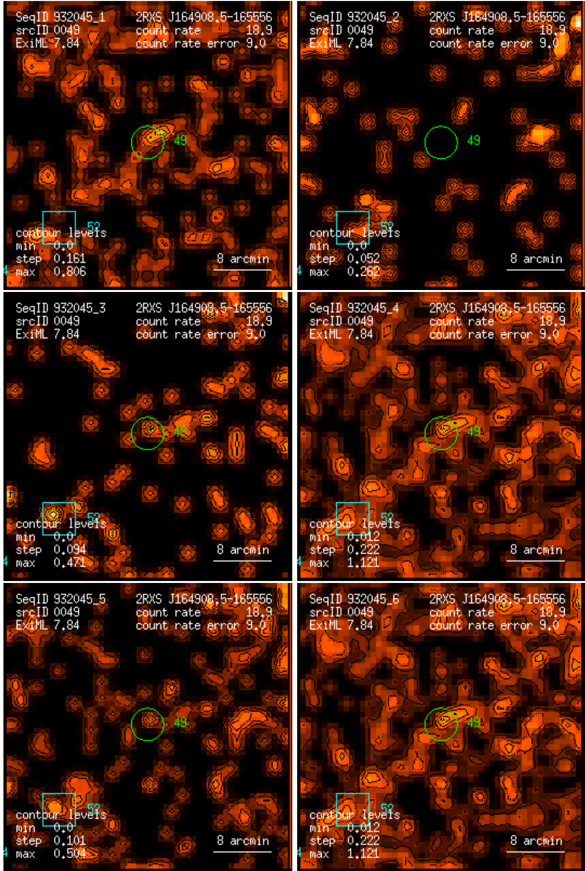
Figure 49: RASS 932045: detection 0049: band rate images, Gaussian filter: (1) PSPC channels 11 – 41, (2) 52 – 90, (3) 91 – 201, (4) 11 – 235, (5) 52 – 201, (6) 11 – 201. Broad band rates in counts/ks. Band rate contour levels in counts/ks/arcmin 2 .
