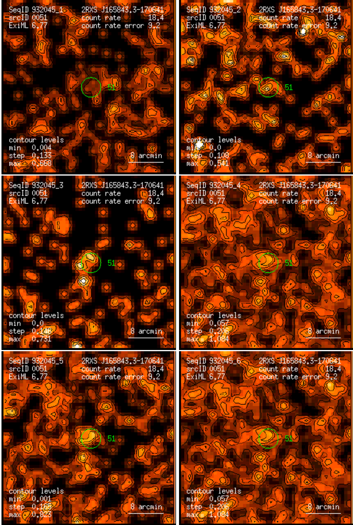
Figure 51: RASS 932045: detection 0051: band rate images, Gaussian filter: (1) PSPC channels 11 – 41, (2) 52 – 90, (3) 91 – 201, (4) 11 – 235, (5) 52 – 201, (6) 11 – 201. Broad band rates in counts/ks. Band rate contour levels in counts/ks/arcmin 2 .
