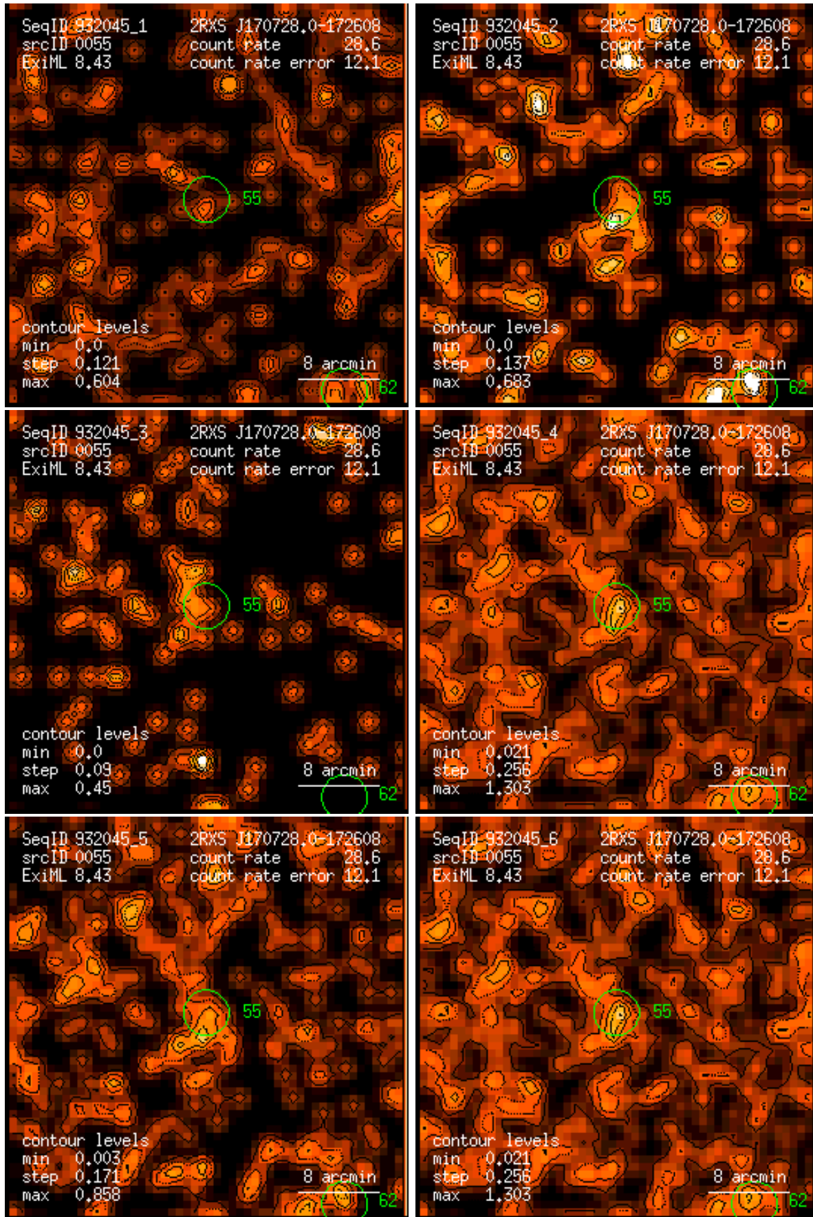
Figure 55: RASS 932045: detection 0055: band rate images, Gaussian filter: (1) PSPC channels 11 – 41, (2) 52 – 90, (3) 91 – 201, (4) 11 – 235, (5) 52 – 201, (6) 11 – 201. Broad band rates in counts/ks. Band rate contour levels in counts/ks/arcmin 2 .
