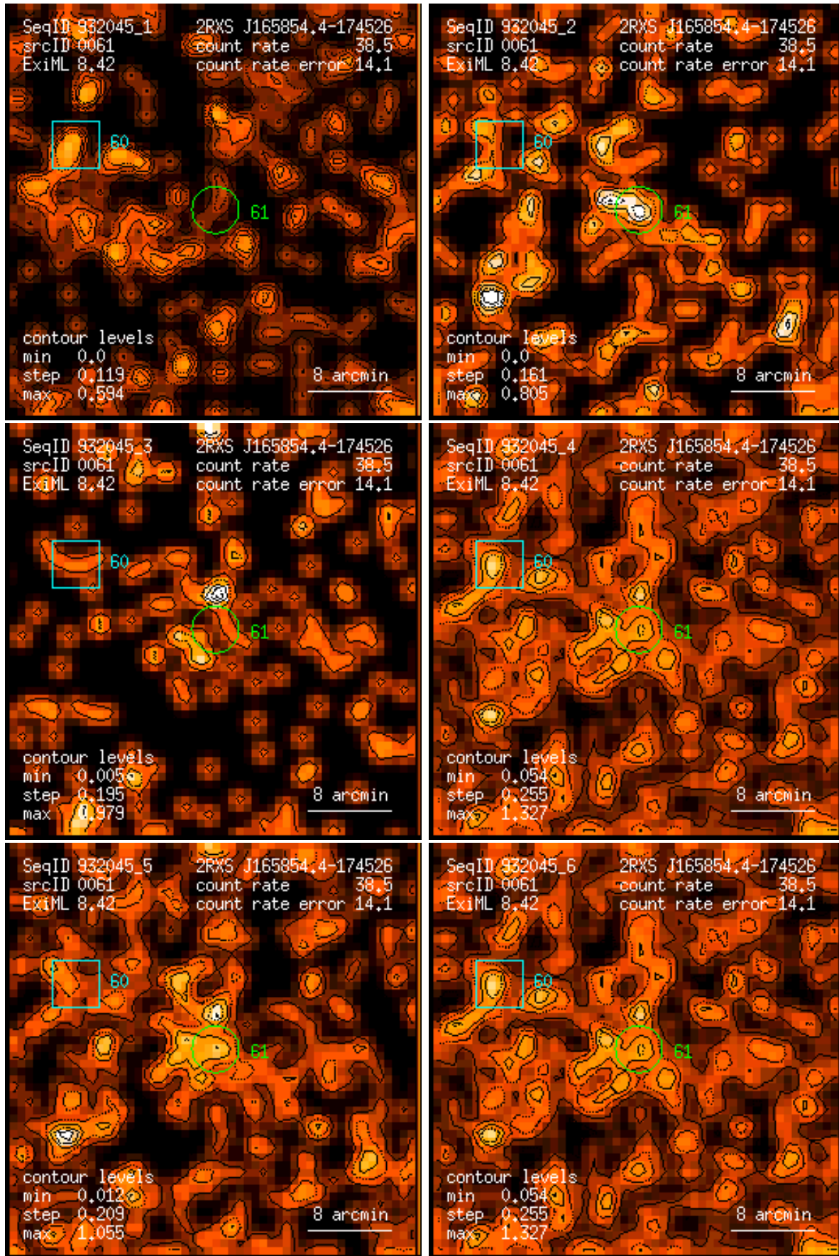
Figure 61: RASS 932045: detection 0061: band rate images, Gaussian filter: (1) PSPC channels 11 – 41, (2) 52 – 90, (3) 91 – 201, (4) 11 – 235, (5) 52 – 201, (6) 11 – 201. Broad band rates in counts/ks. Band rate contour levels in counts/ks/arcmin 2 .
