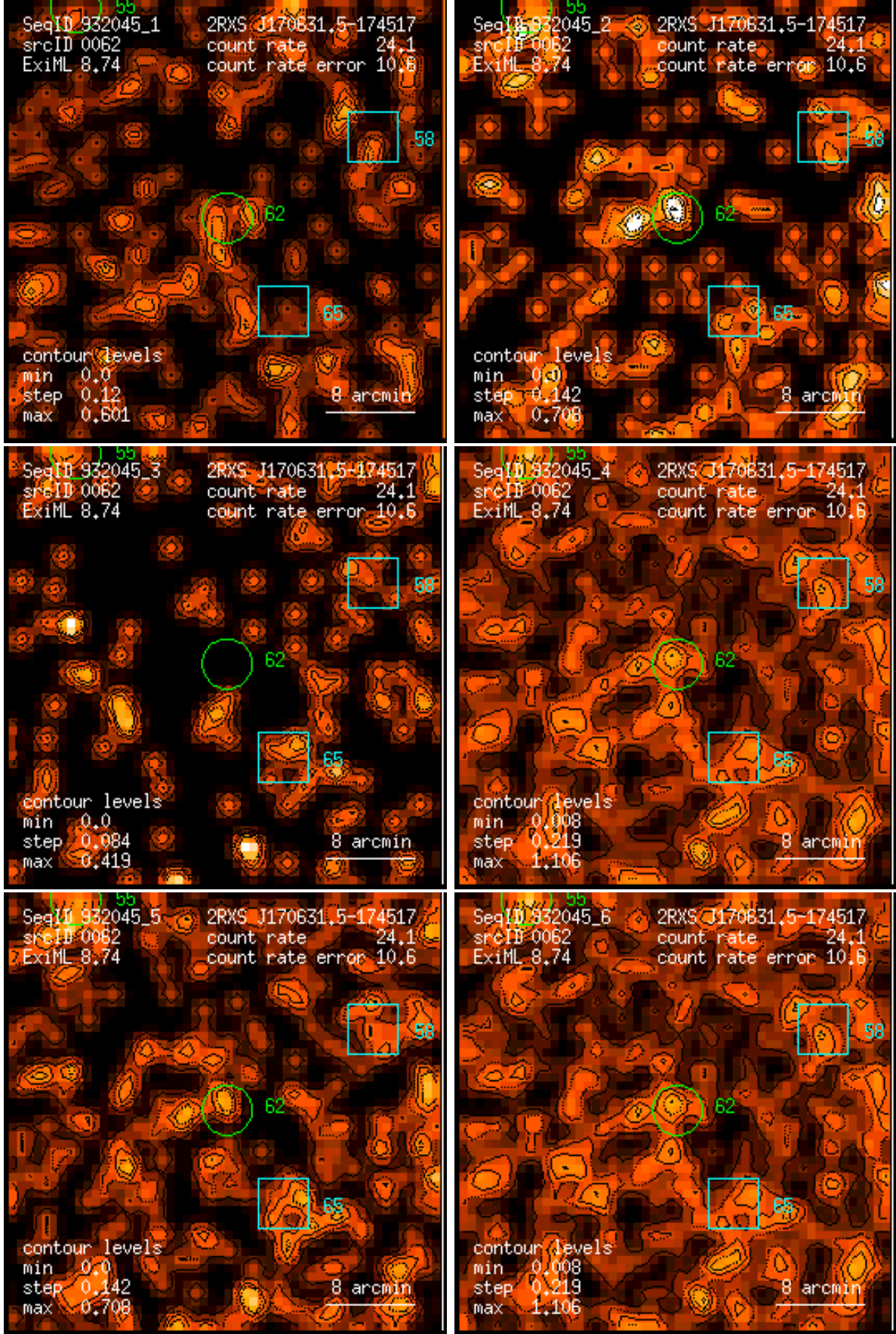
Figure 62: RASS 932045: detection 0062: band rate images, Gaussian filter: (1) PSPC channels 11 – 41, (2) 52 – 90, (3) 91 – 201, (4) 11 – 235, (5) 52 – 201, (6) 11 – 201. Broad band rates in counts/ks. Band rate contour levels in counts/ks/arcmin 2 .
