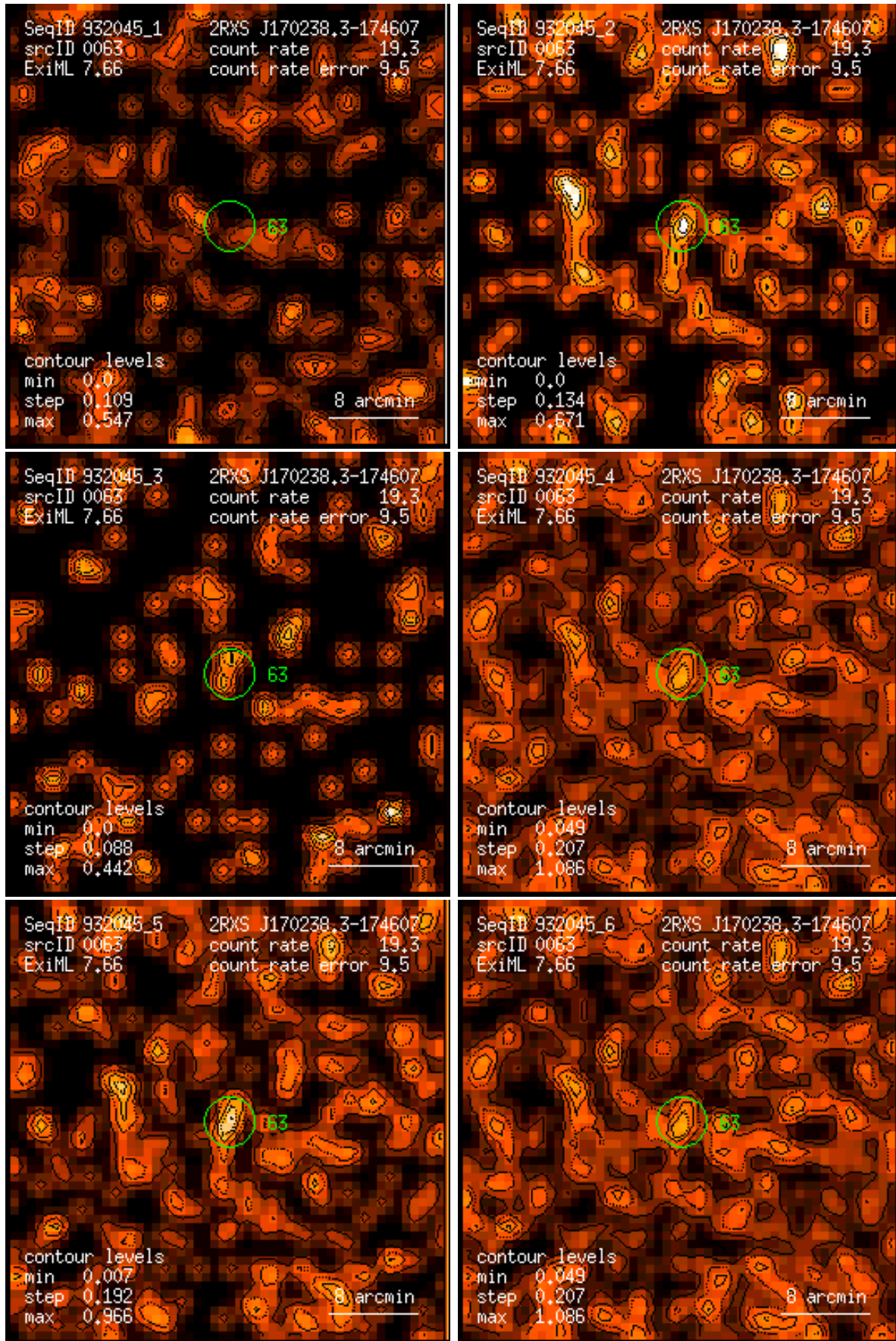
Figure 63: RASS 932045: detection 0063: band rate images, Gaussian filter: (1) PSPC channels 11 – 41, (2) 52 – 90, (3) 91 – 201, (4) 11 – 235, (5) 52 – 201, (6) 11 – 201. Broad band rates in counts/ks. Band rate contour levels in counts/ks/arcmin 2 .
