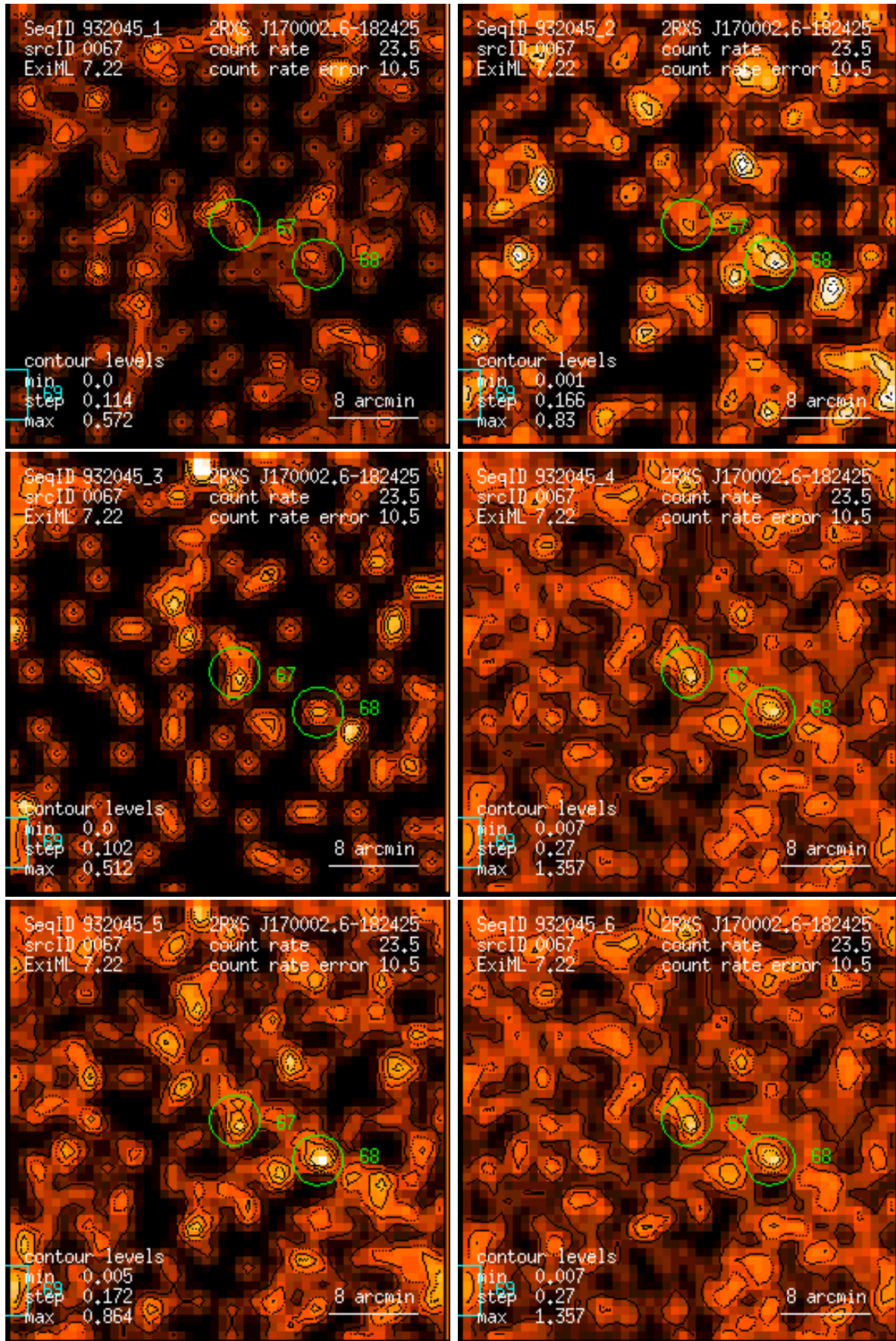
Figure 67: RASS 932045: detection 0067: band rate images, Gaussian filter: (1) PSPC channels 11 – 41, (2) 52 – 90, (3) 91 – 201, (4) 11 – 235, (5) 52 – 201, (6) 11 – 201. Broad band rates in counts/ks. Band rate contour levels in counts/ks/arcmin 2 .
