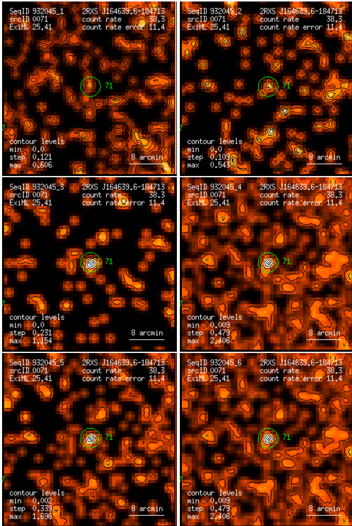
Figure 71: RASS 932045: detection 0071: band rate images, Gaussian filter: (1) PSPC channels 11 – 41, (2) 52 – 90, (3) 91 – 201, (4) 11 – 235, (5) 52 – 201, (6) 11 – 201. Broad band rates in counts/ks. Band rate contour levels in counts/ks/arcmin 2 .
