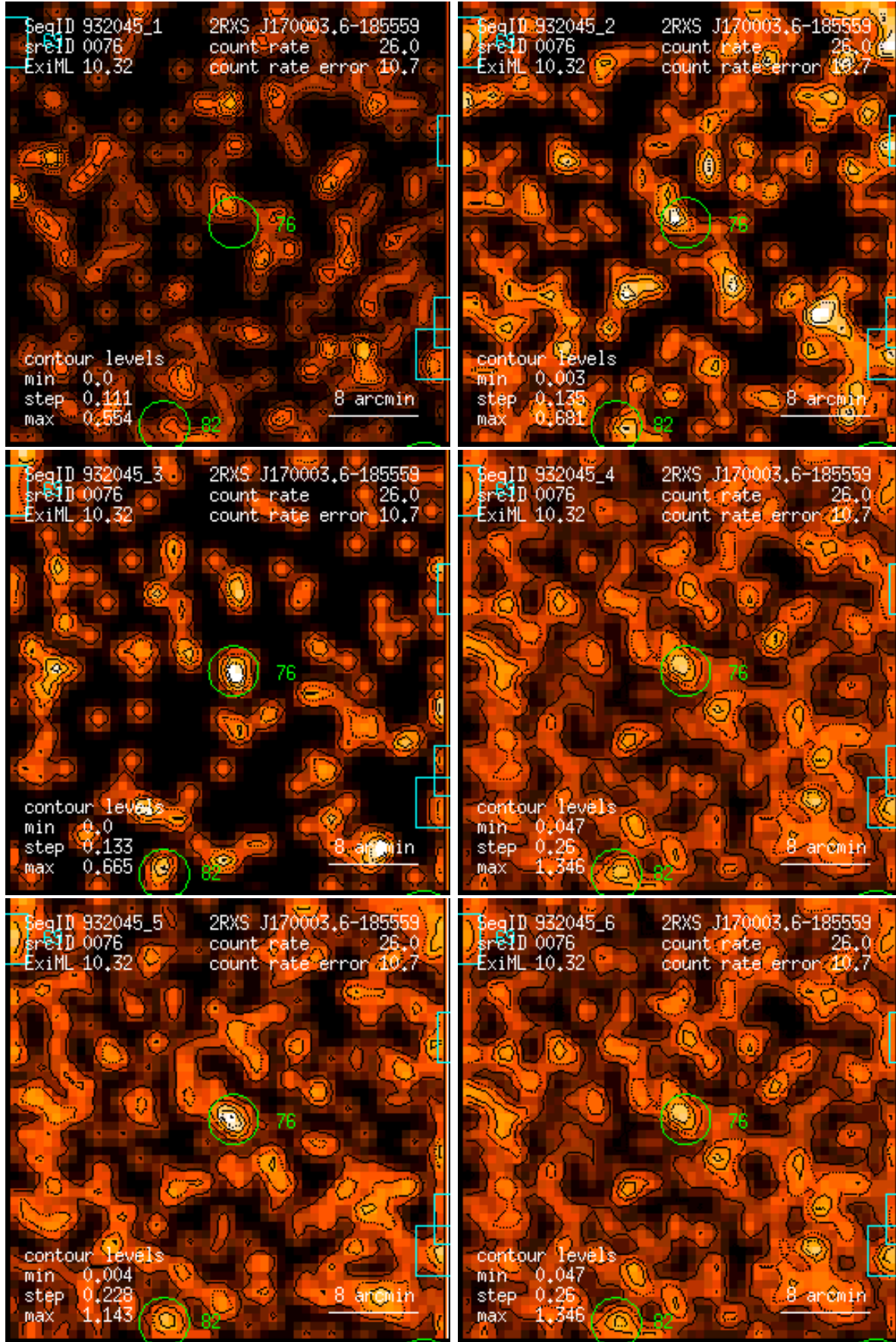
Figure 76: RASS 932045: detection 0076: band rate images, Gaussian filter: (1) PSPC channels 11 – 41, (2) 52 – 90, (3) 91 – 201, (4) 11 – 235, (5) 52 – 201, (6) 11 – 201. Broad band rates in counts/ks. Band rate contour levels in counts/ks/arcmin 2 .
