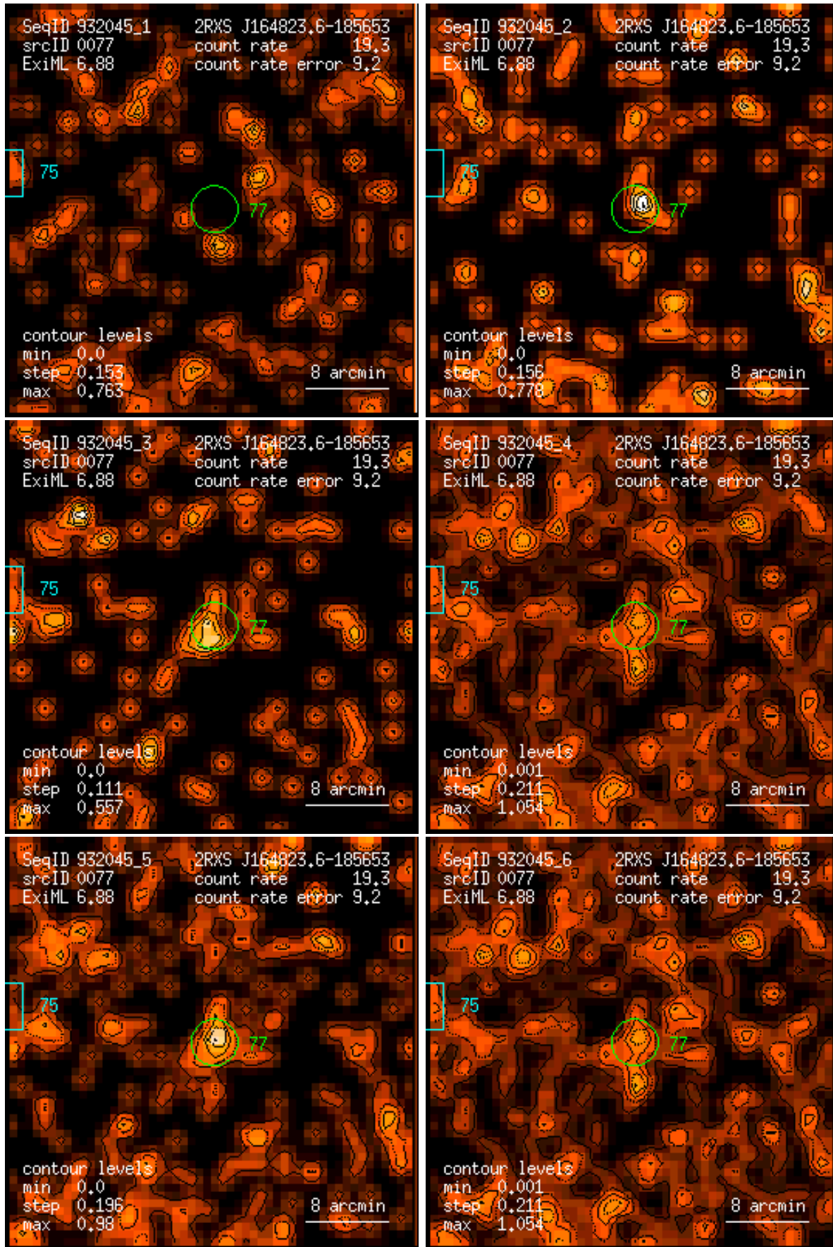
Figure 77: RASS 932045: detection 0077: band rate images, Gaussian filter: (1) PSPC channels 11 – 41, (2) 52 – 90, (3) 91 – 201, (4) 11 – 235, (5) 52 – 201, (6) 11 – 201. Broad band rates in counts/ks. Band rate contour levels in counts/ks/arcmin 2 .
