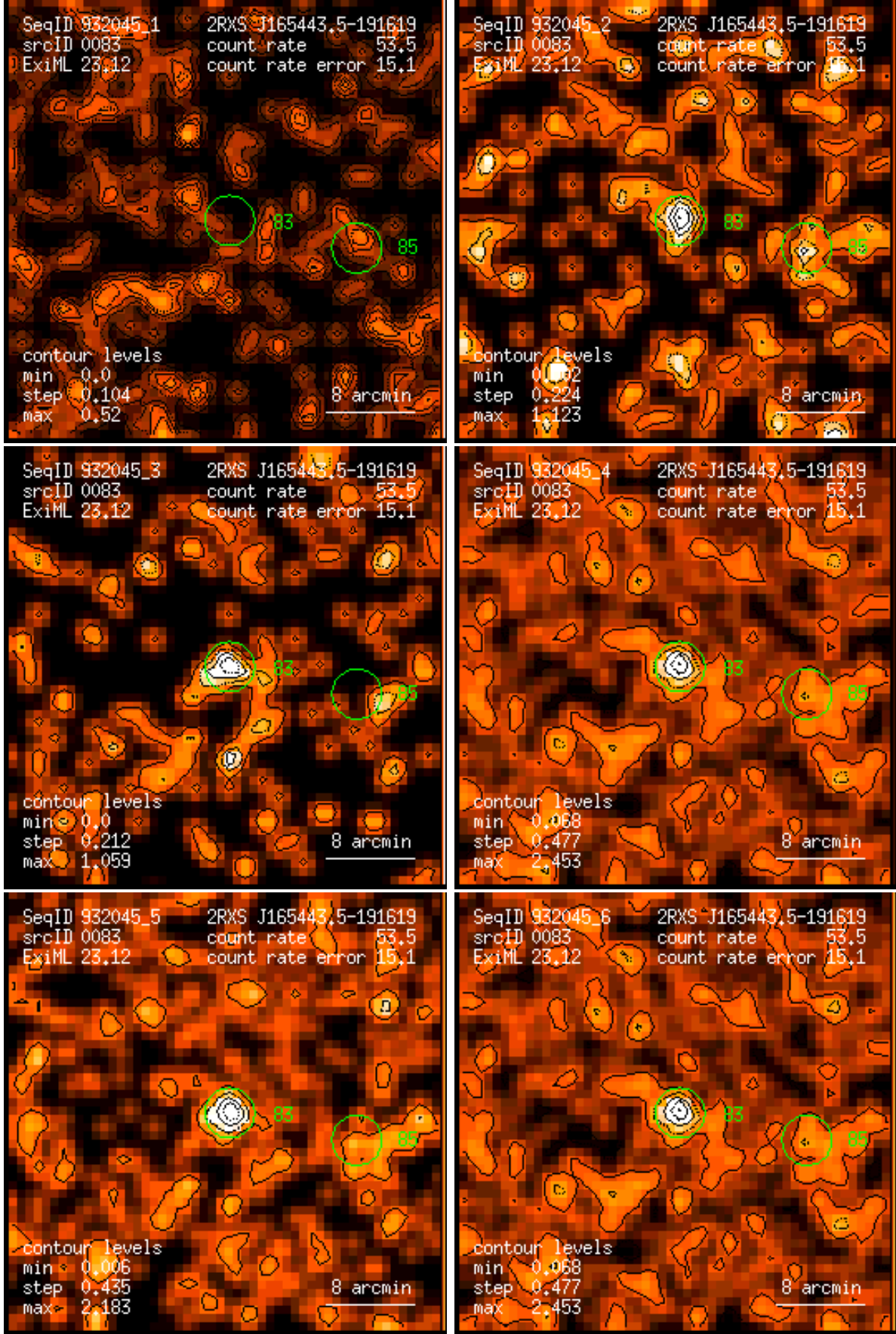
Figure 83: RASS 932045: detection 0083: band rate images, Gaussian filter: (1) PSPC channels 11 – 41, (2) 52 – 90, (3) 91 – 201, (4) 11 – 235, (5) 52 – 201, (6) 11 – 201. Broad band rates in counts/ks. Band rate contour levels in counts/ks/arcmin 2 .
