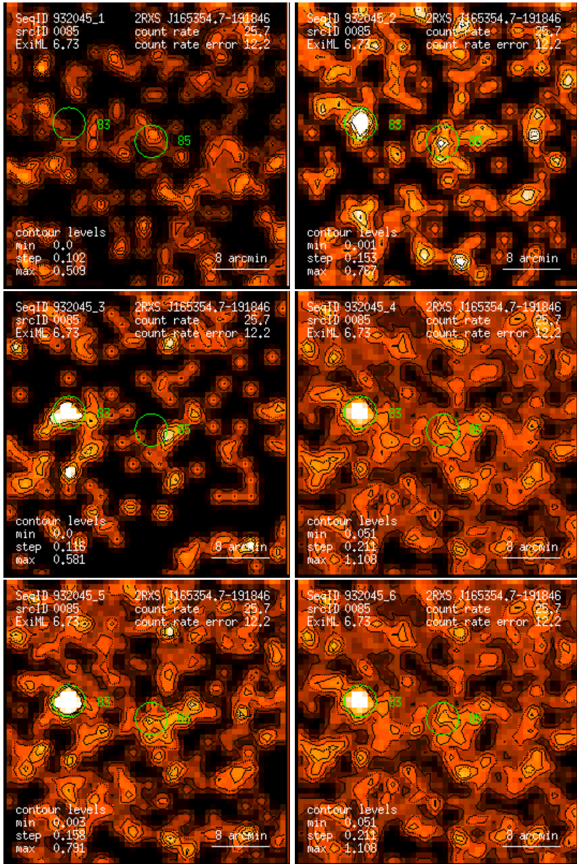
Figure 85: RASS 932045: detection 0085: band rate images, Gaussian filter: (1) PSPC channels 11 – 41, (2) 52 – 90, (3) 91 – 201, (4) 11 – 235, (5) 52 – 201, (6) 11 – 201. Broad band rates in counts/ks. Band rate contour levels in counts/ks/arcmin 2 .
