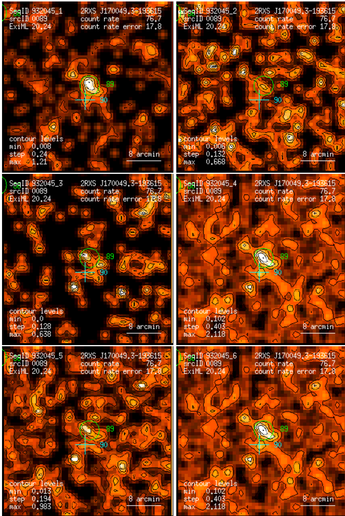
Figure 89: RASS 932045: detection 0089: band rate images, Gaussian filter: (1) PSPC channels 11 – 41, (2) 52 – 90, (3) 91 – 201, (4) 11 – 235, (5) 52 – 201, (6) 11 – 201. Broad band rates in counts/ks. Band rate contour levels in counts/ks/arcmin 2 .
