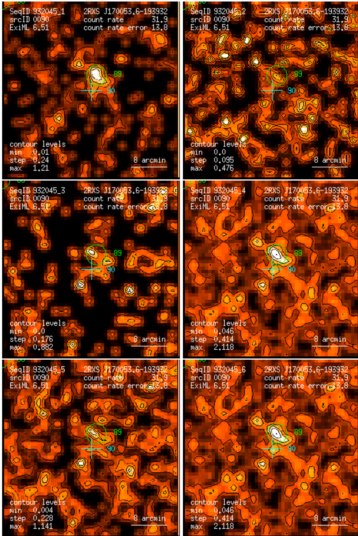
Figure 90: RASS 932045: detection 0090: band rate images, Gaussian filter: (1) PSPC channels 11 – 41, (2) 52 – 90, (3) 91 – 201, (4) 11 – 235, (5) 52 – 201, (6) 11 – 201. Broad band rates in counts/ks. Band rate contour levels in counts/ks/arcmin 2 .
