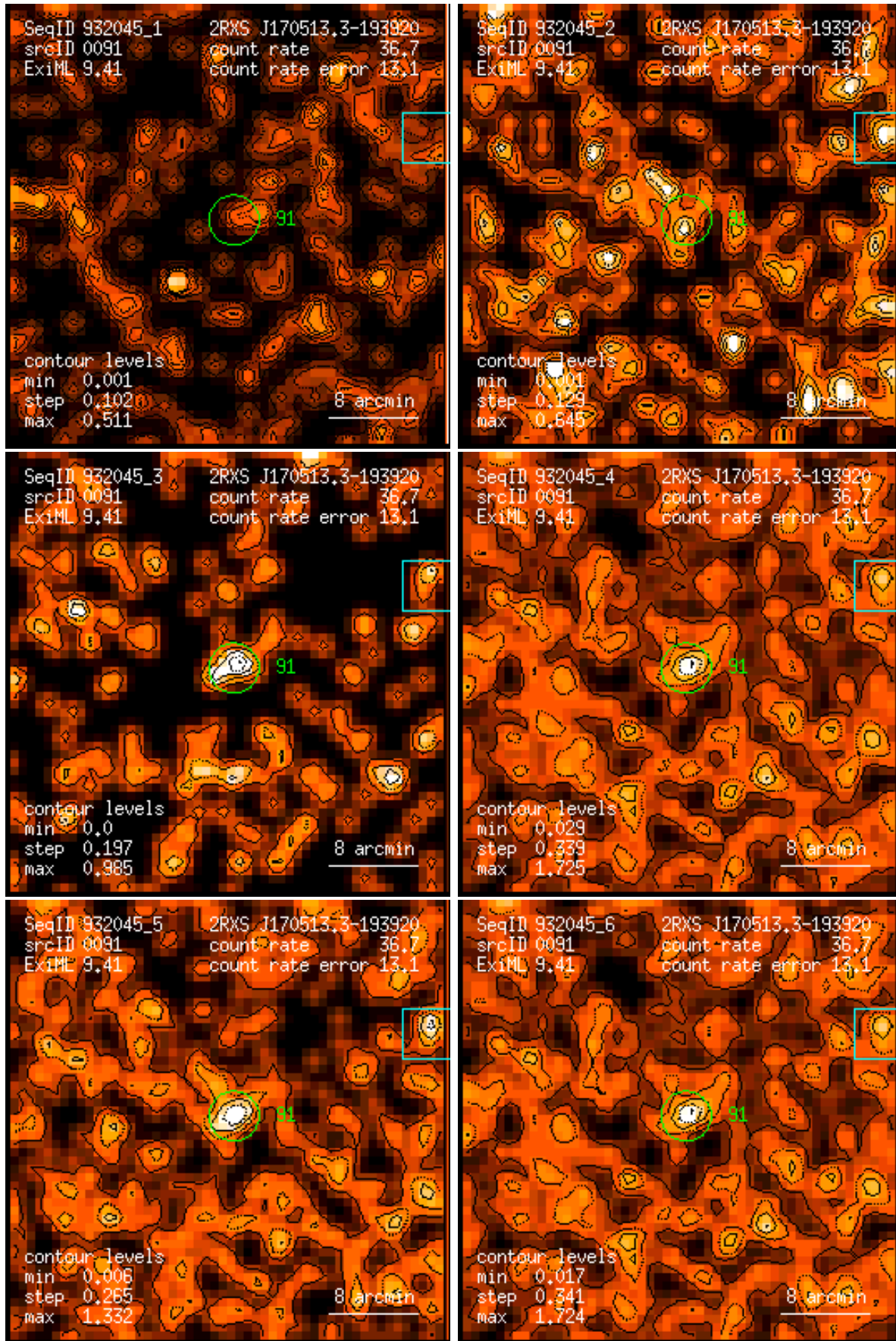
Figure 91: RASS 932045: detection 0091: band rate images, Gaussian filter: (1) PSPC channels 11 – 41, (2) 52 – 90, (3) 91 – 201, (4) 11 – 235, (5) 52 – 201, (6) 11 – 201. Broad band rates in counts/ks. Band rate contour levels in counts/ks/arcmin 2 .
