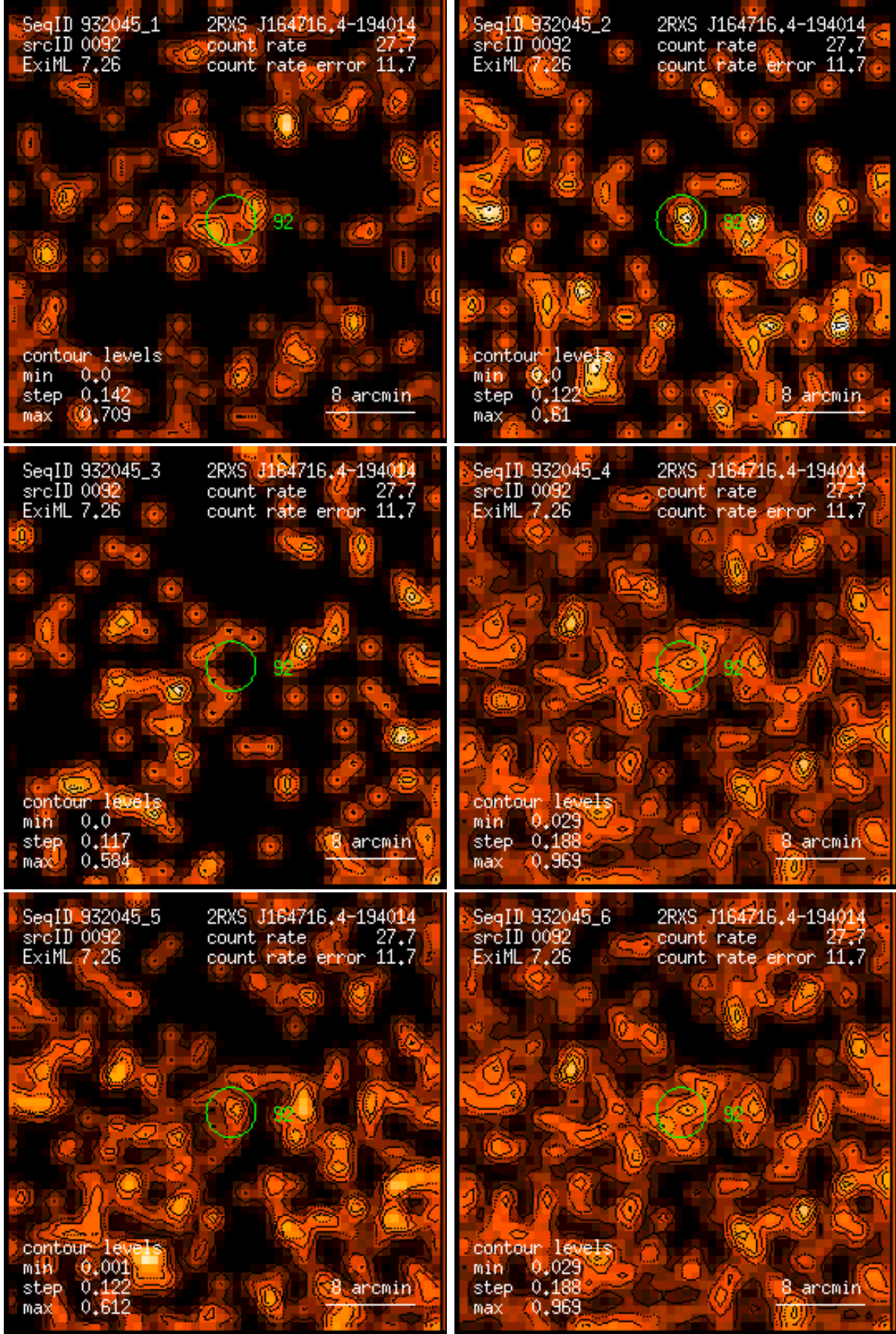
Figure 92: RASS 932045: detection 0092: band rate images, Gaussian filter: (1) PSPC channels 11 – 41, (2) 52 – 90, (3) 91 – 201, (4) 11 – 235, (5) 52 – 201, (6) 11 – 201. Broad band rates in counts/ks. Band rate contour levels in counts/ks/arcmin 2 .
