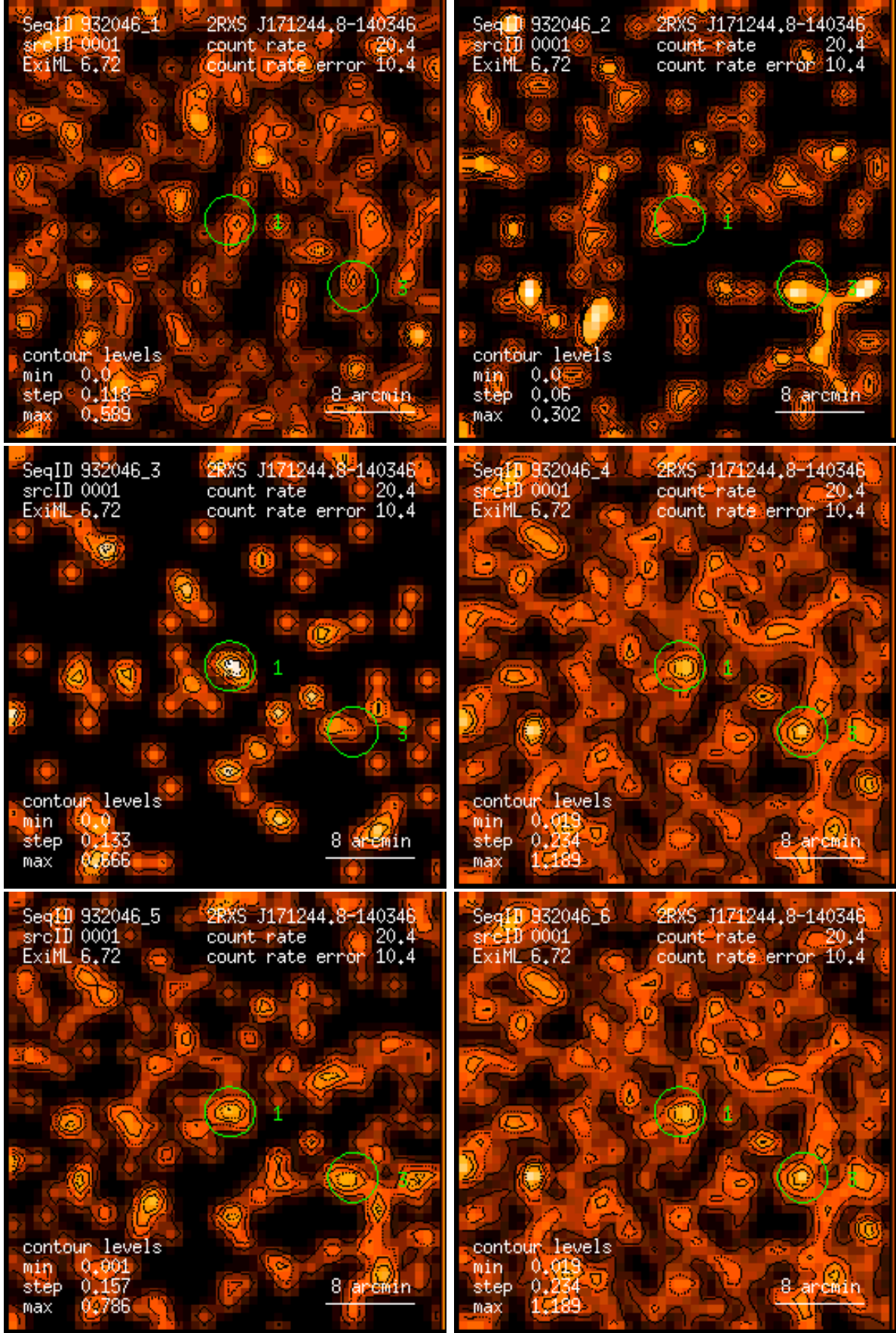
Figure 1: RASS 932046: detection 0001: band rate images, Gaussian filter: (1) PSPC channels 11 – 41, (2) 52 – 90, (3) 91 – 201, (4) 11 – 235, (5) 52 – 201, (6) 11 – 201. Broad band rates in counts/ks. Band rate contour levels in counts/ks/arcmin 2 .
