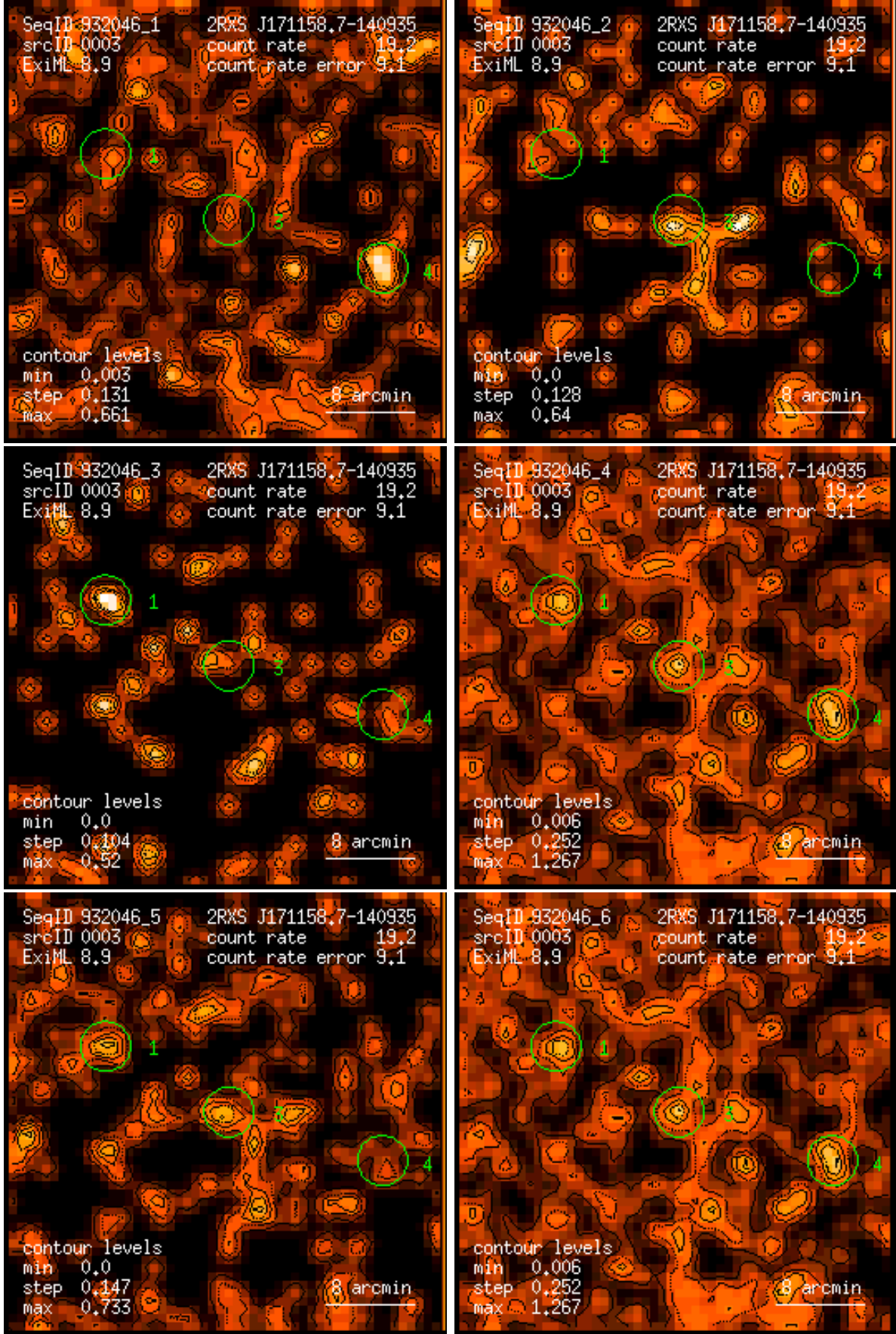
Figure 3: RASS 932046: detection 0003: band rate images, Gaussian filter: (1) PSPC channels 11 – 41, (2) 52 – 90, (3) 91 – 201, (4) 11 – 235, (5) 52 – 201, (6) 11 – 201. Broad band rates in counts/ks. Band rate contour levels in counts/ks/arcmin 2 .
