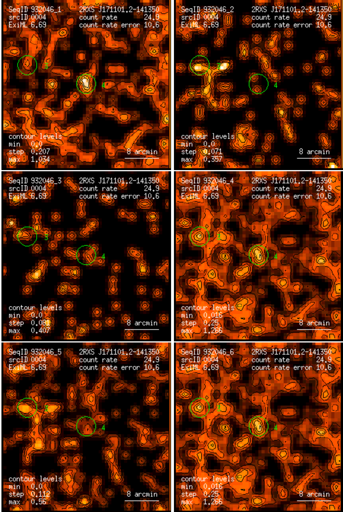
Figure 4: RASS 932046: detection 0004: band rate images, Gaussian filter: (1) PSPC channels 11 – 41, (2) 52 – 90, (3) 91 – 201, (4) 11 – 235, (5) 52 – 201, (6) 11 – 201. Broad band rates in counts/ks. Band rate contour levels in counts/ks/arcmin 2 .
