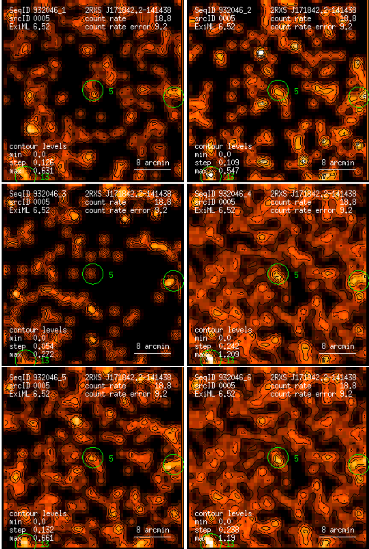
Figure 5: RASS 932046: detection 0005: band rate images, Gaussian filter: (1) PSPC channels 11 – 41, (2) 52 – 90, (3) 91 – 201, (4) 11 – 235, (5) 52 – 201, (6) 11 – 201. Broad band rates in counts/ks. Band rate contour levels in counts/ks/arcmin 2 .
