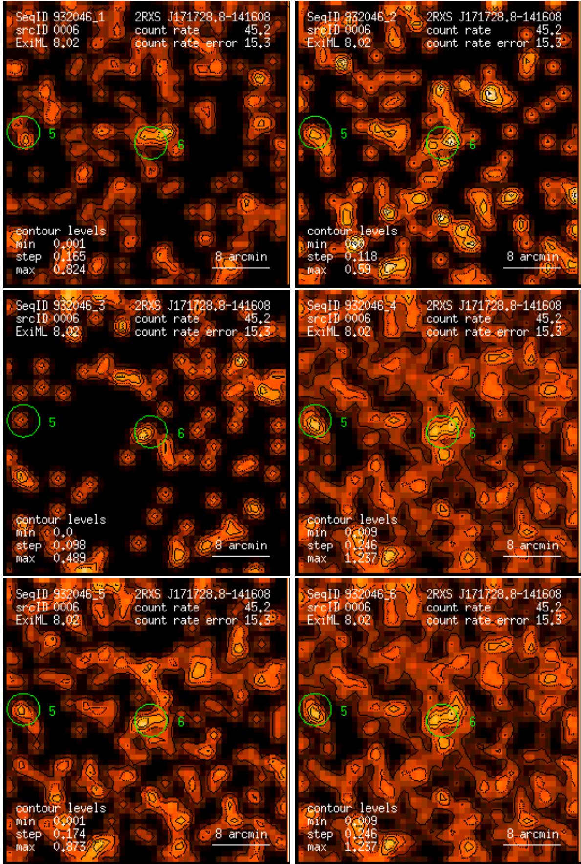
Figure 6: RASS 932046: detection 0006: band rate images, Gaussian filter: (1) PSPC channels 11 – 41, (2) 52 – 90, (3) 91 – 201, (4) 11 – 235, (5) 52 – 201, (6) 11 – 201. Broad band rates in counts/ks. Band rate contour levels in counts/ks/arcmin 2 .
