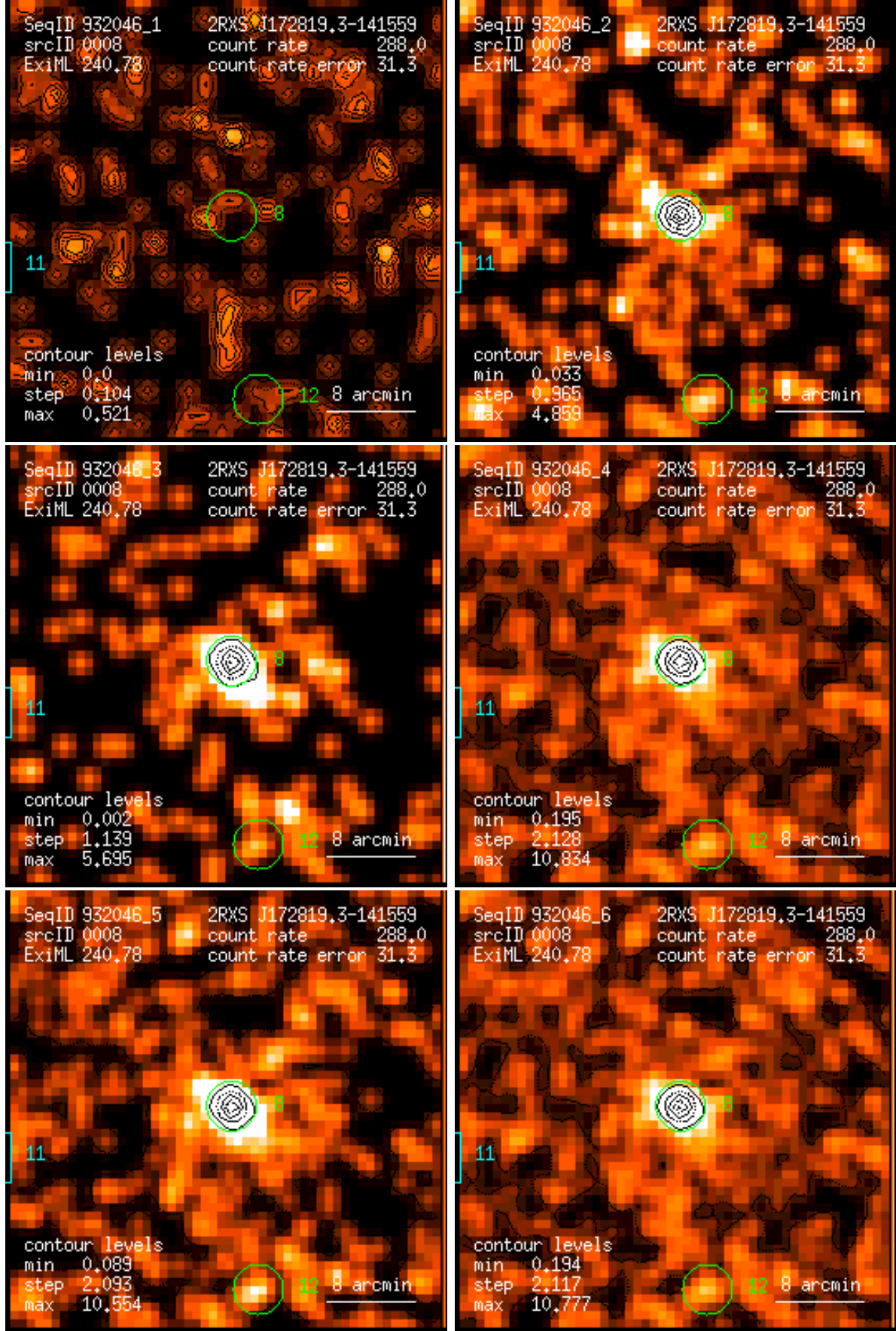
Figure 8: RASS 932046: detection 0008: band rate images, Gaussian filter: (1) PSPC channels 11 – 41, (2) 52 – 90, (3) 91 – 201, (4) 11 – 235, (5) 52 – 201, (6) 11 – 201. Broad band rates in counts/ks. Band rate contour levels in counts/ks/arcmin 2 .
