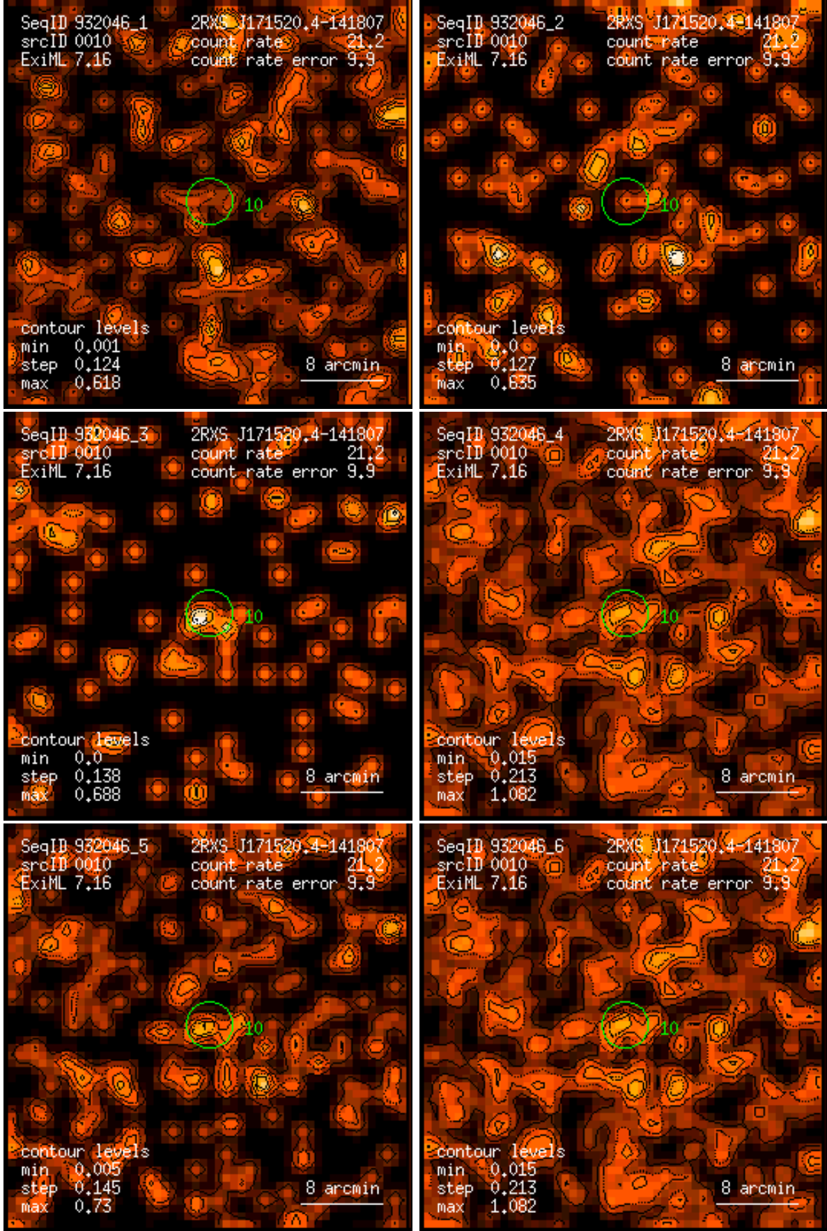
Figure 10: RASS 932046: detection 0010: band rate images, Gaussian filter: (1) PSPC channels 11 – 41, (2) 52 – 90, (3) 91 – 201, (4) 11 – 235, (5) 52 – 201, (6) 11 – 201. Broad band rates in counts/ks. Band rate contour levels in counts/ks/arcmin 2 .
