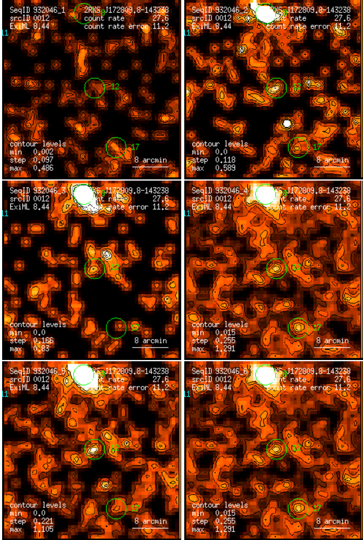
Figure 12: RASS 932046: detection 0012: band rate images, Gaussian filter: (1) PSPC channels 11 – 41, (2) 52 – 90, (3) 91 – 201, (4) 11 – 235, (5) 52 – 201, (6) 11 – 201. Broad band rates in counts/ks. Band rate contour levels in counts/ks/arcmin 2 .
