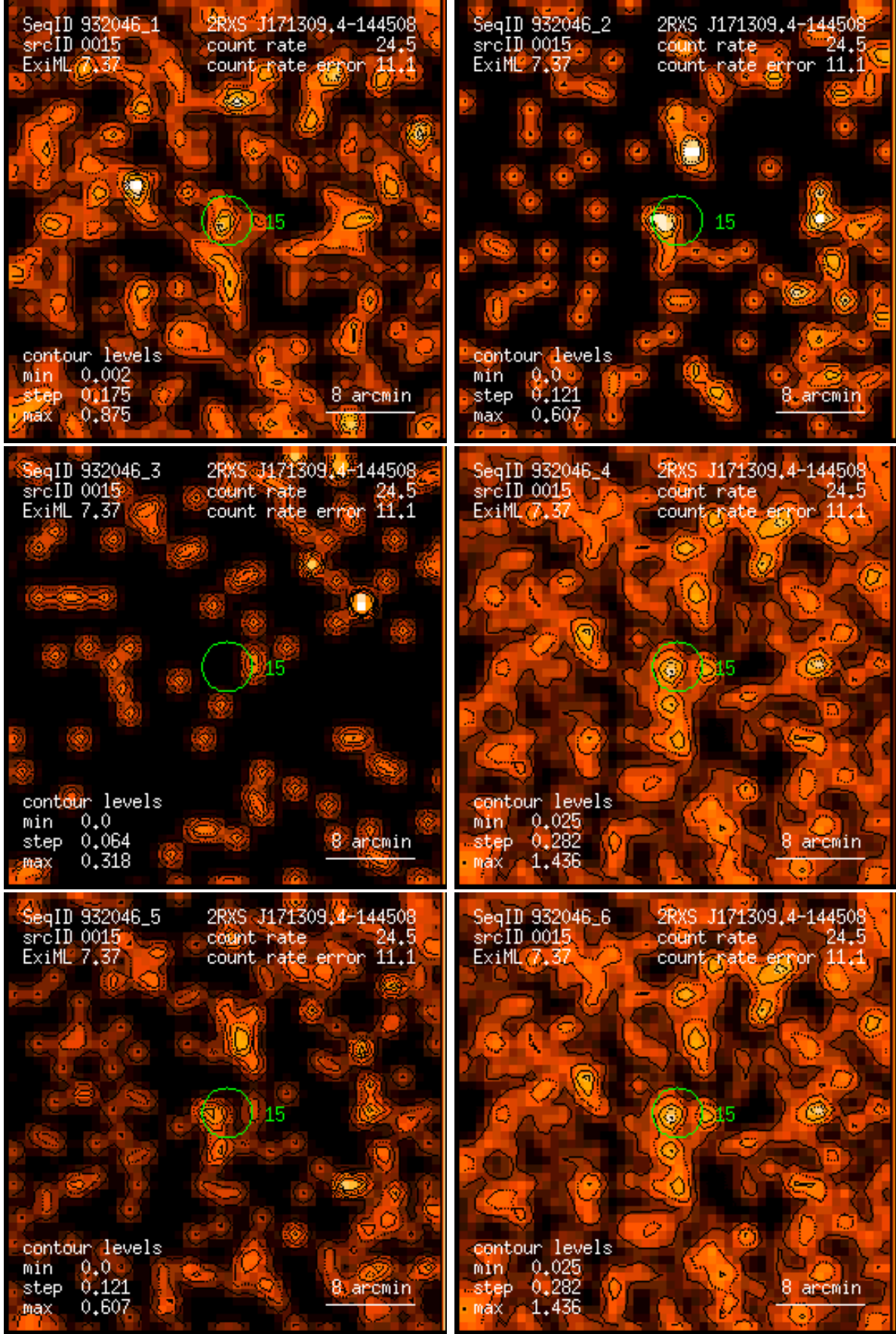
Figure 15: RASS 932046: detection 0015: band rate images, Gaussian filter: (1) PSPC channels 11 – 41, (2) 52 – 90, (3) 91 – 201, (4) 11 – 235, (5) 52 – 201, (6) 11 – 201. Broad band rates in counts/ks. Band rate contour levels in counts/ks/arcmin 2 .
