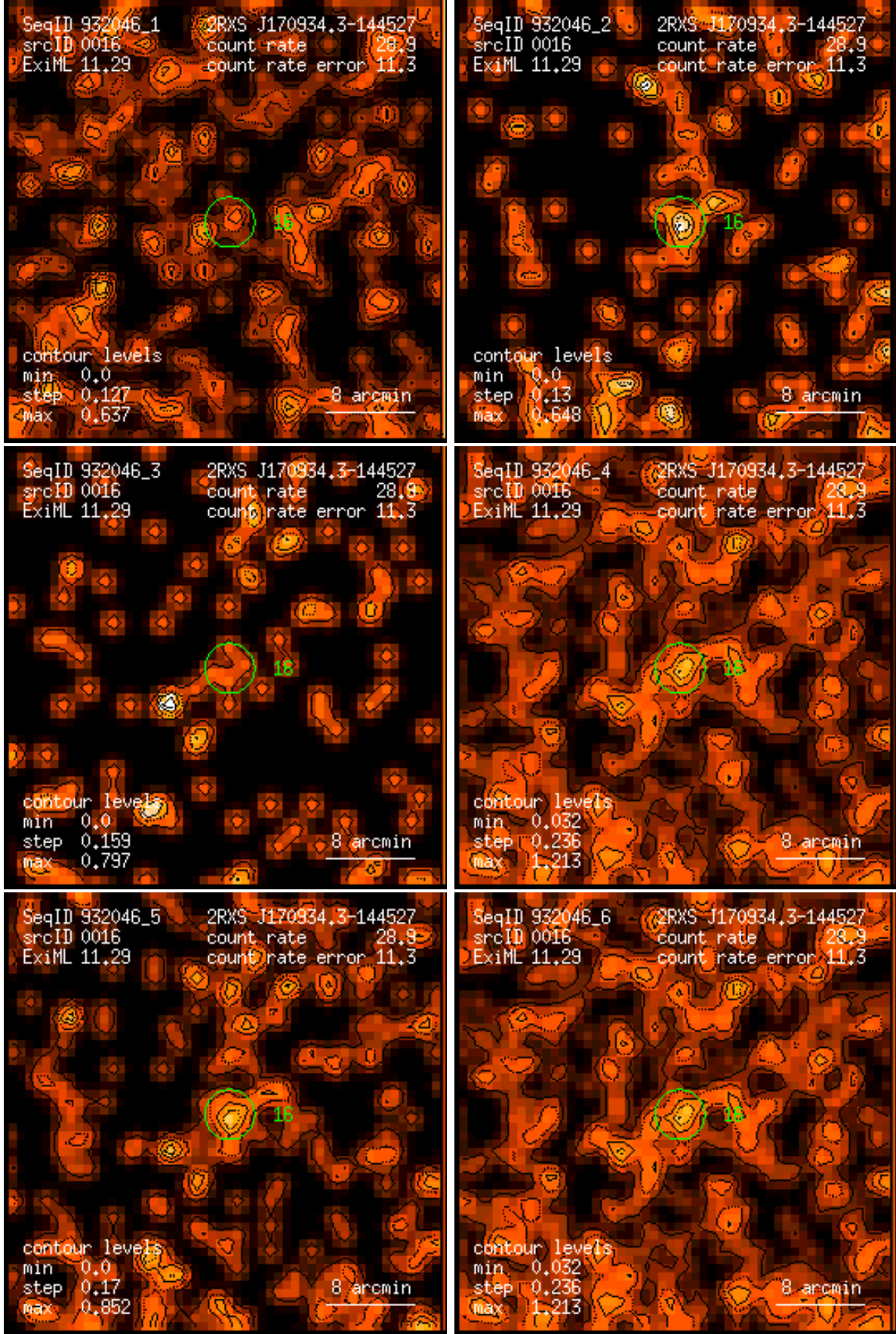
Figure 16: RASS 932046: detection 0016: band rate images, Gaussian filter: (1) PSPC channels 11 – 41, (2) 52 – 90, (3) 91 – 201, (4) 11 – 235, (5) 52 – 201, (6) 11 – 201. Broad band rates in counts/ks. Band rate contour levels in counts/ks/arcmin 2 .
