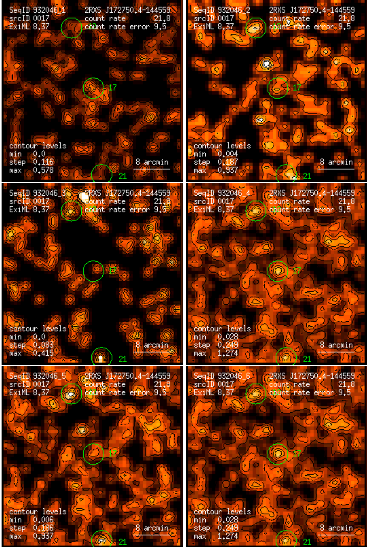
Figure 17: RASS 932046: detection 0017: band rate images, Gaussian filter: (1) PSPC channels 11 – 41, (2) 52 – 90, (3) 91 – 201, (4) 11 – 235, (5) 52 – 201, (6) 11 – 201. Broad band rates in counts/ks. Band rate contour levels in counts/ks/arcmin 2 .
