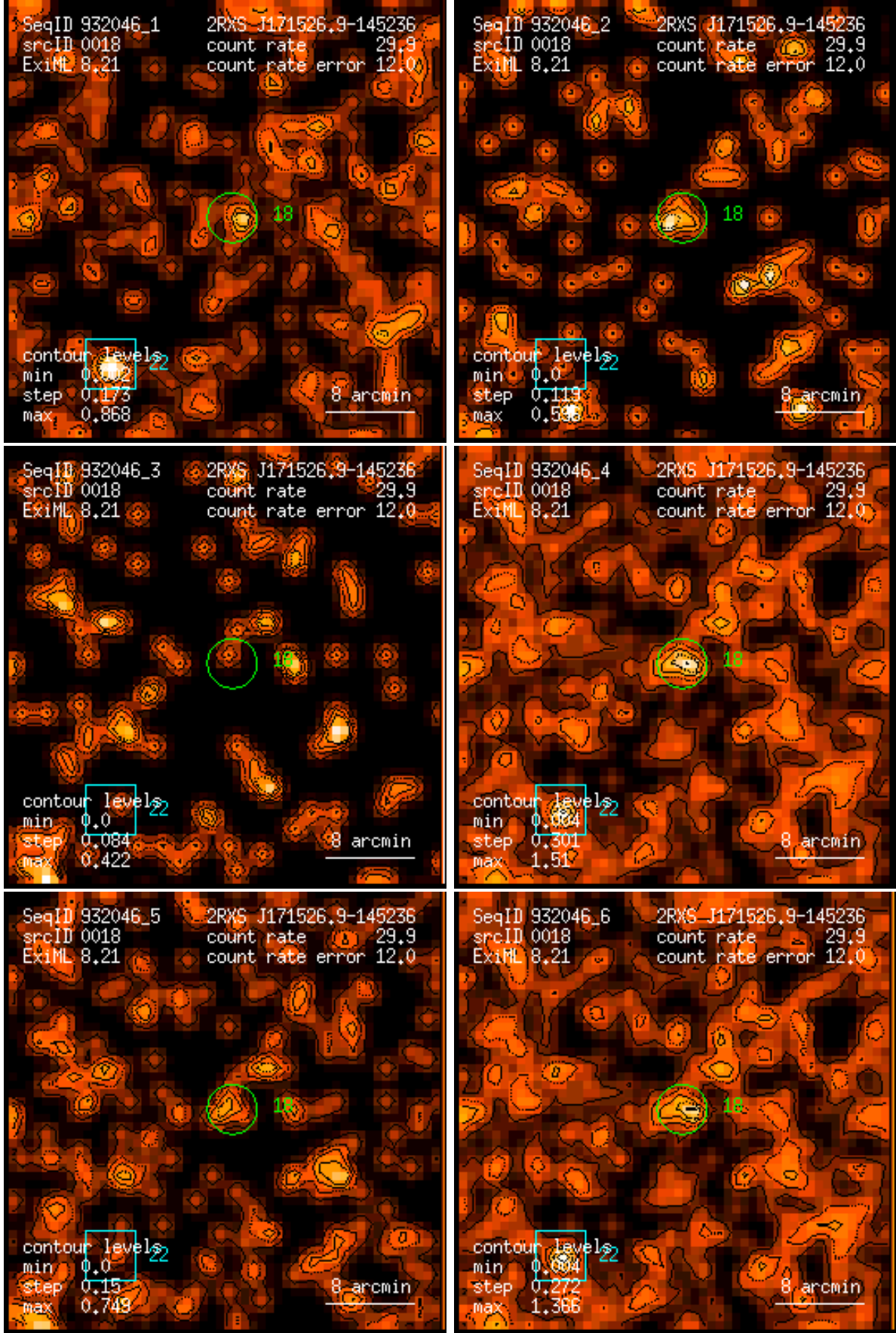
Figure 18: RASS 932046: detection 0018: band rate images, Gaussian filter: (1) PSPC channels 11 – 41, (2) 52 – 90, (3) 91 – 201, (4) 11 – 235, (5) 52 – 201, (6) 11 – 201. Broad band rates in counts/ks. Band rate contour levels in counts/ks/arcmin 2 .
