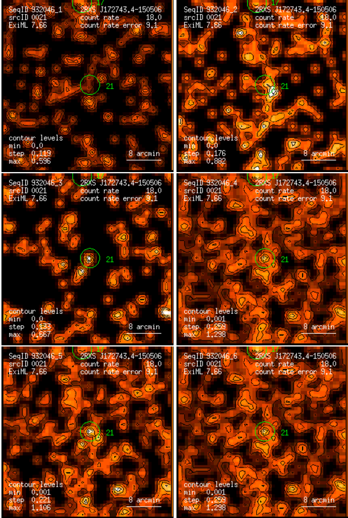
Figure 21: RASS 932046: detection 0021: band rate images, Gaussian filter: (1) PSPC channels 11 – 41, (2) 52 – 90, (3) 91 – 201, (4) 11 – 235, (5) 52 – 201, (6) 11 – 201. Broad band rates in counts/ks. Band rate contour levels in counts/ks/arcmin 2 .
