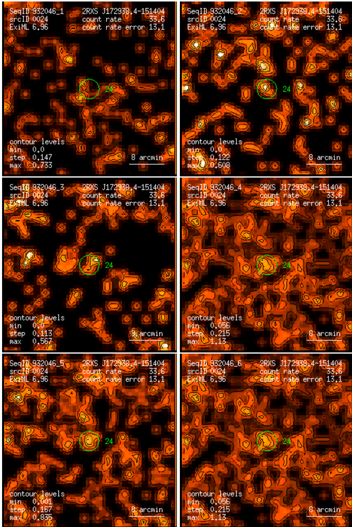
Figure 24: RASS 932046: detection 0024: band rate images, Gaussian filter: (1) PSPC channels 11 – 41, (2) 52 – 90, (3) 91 – 201, (4) 11 – 235, (5) 52 – 201, (6) 11 – 201. Broad band rates in counts/ks. Band rate contour levels in counts/ks/arcmin 2 .
