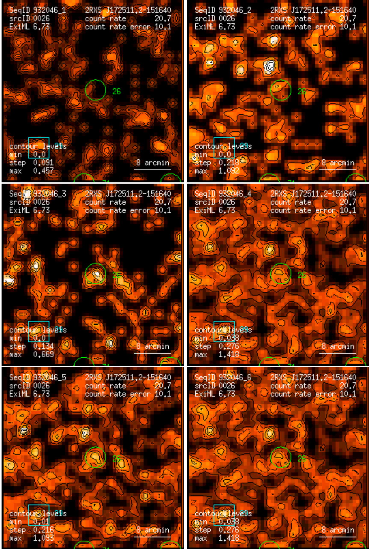
Figure 26: RASS 932046: detection 0026: band rate images, Gaussian filter: (1) PSPC channels 11 – 41, (2) 52 – 90, (3) 91 – 201, (4) 11 – 235, (5) 52 – 201, (6) 11 – 201. Broad band rates in counts/ks. Band rate contour levels in counts/ks/arcmin 2 .
