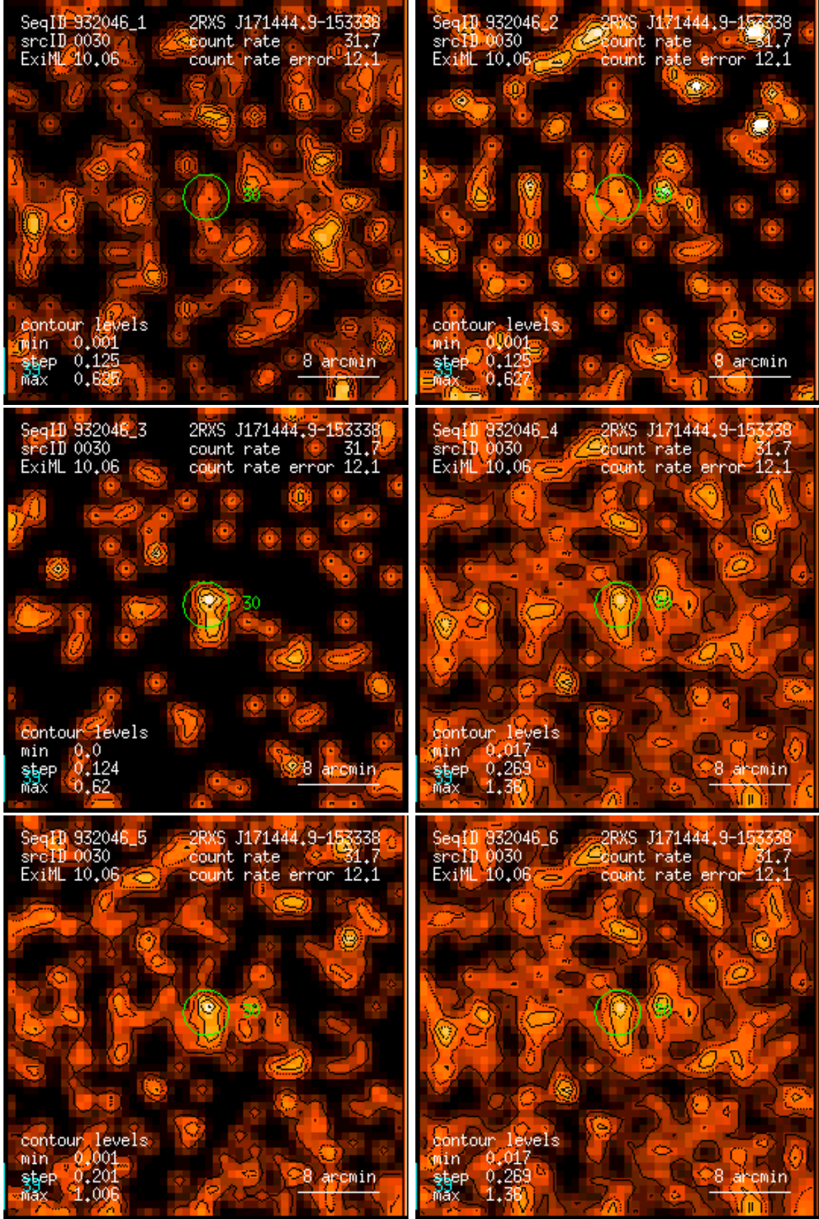
Figure 30: RASS 932046: detection 0030: band rate images, Gaussian filter: (1) PSPC channels 11 – 41, (2) 52 – 90, (3) 91 – 201, (4) 11 – 235, (5) 52 – 201, (6) 11 – 201. Broad band rates in counts/ks. Band rate contour levels in counts/ks/arcmin 2 .
