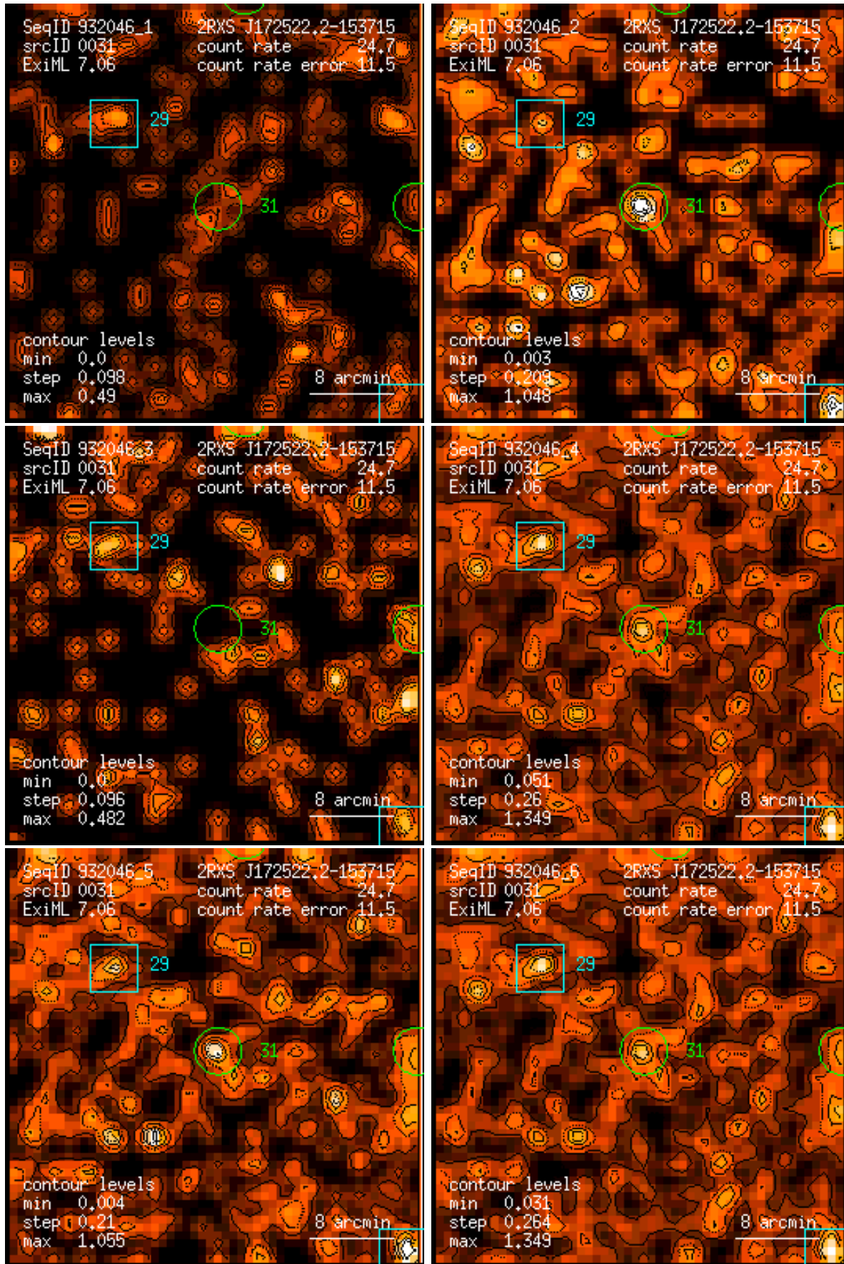
Figure 31: RASS 932046: detection 0031: band rate images, Gaussian filter: (1) PSPC channels 11 – 41, (2) 52 – 90, (3) 91 – 201, (4) 11 – 235, (5) 52 – 201, (6) 11 – 201. Broad band rates in counts/ks. Band rate contour levels in counts/ks/arcmin 2 .
