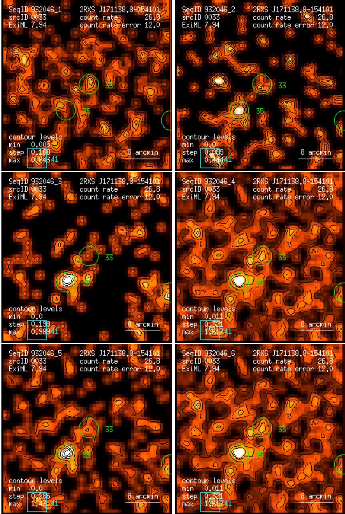
Figure 33: RASS 932046: detection 0033: band rate images, Gaussian filter: (1) PSPC channels 11 – 41, (2) 52 – 90, (3) 91 – 201, (4) 11 – 235, (5) 52 – 201, (6) 11 – 201. Broad band rates in counts/ks. Band rate contour levels in counts/ks/arcmin 2 .
