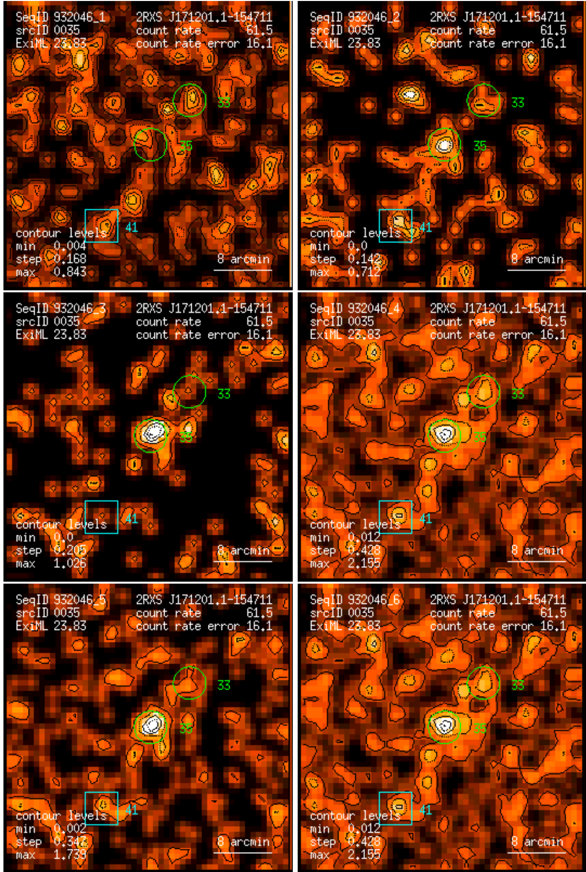
Figure 35: RASS 932046: detection 0035: band rate images, Gaussian filter: (1) PSPC channels 11 – 41, (2) 52 – 90, (3) 91 – 201, (4) 11 – 235, (5) 52 – 201, (6) 11 – 201. Broad band rates in counts/ks. Band rate contour levels in counts/ks/arcmin 2 .
