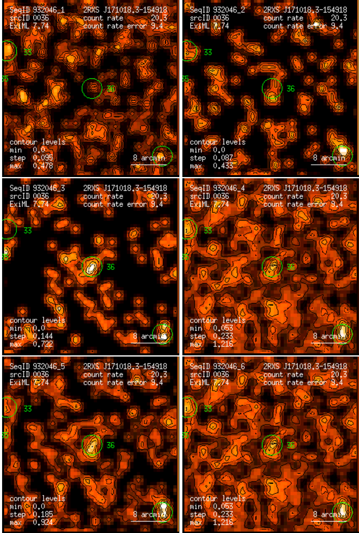
Figure 36: RASS 932046: detection 0036: band rate images, Gaussian filter: (1) PSPC channels 11 – 41, (2) 52 – 90, (3) 91 – 201, (4) 11 – 235, (5) 52 – 201, (6) 11 – 201. Broad band rates in counts/ks. Band rate contour levels in counts/ks/arcmin 2 .
