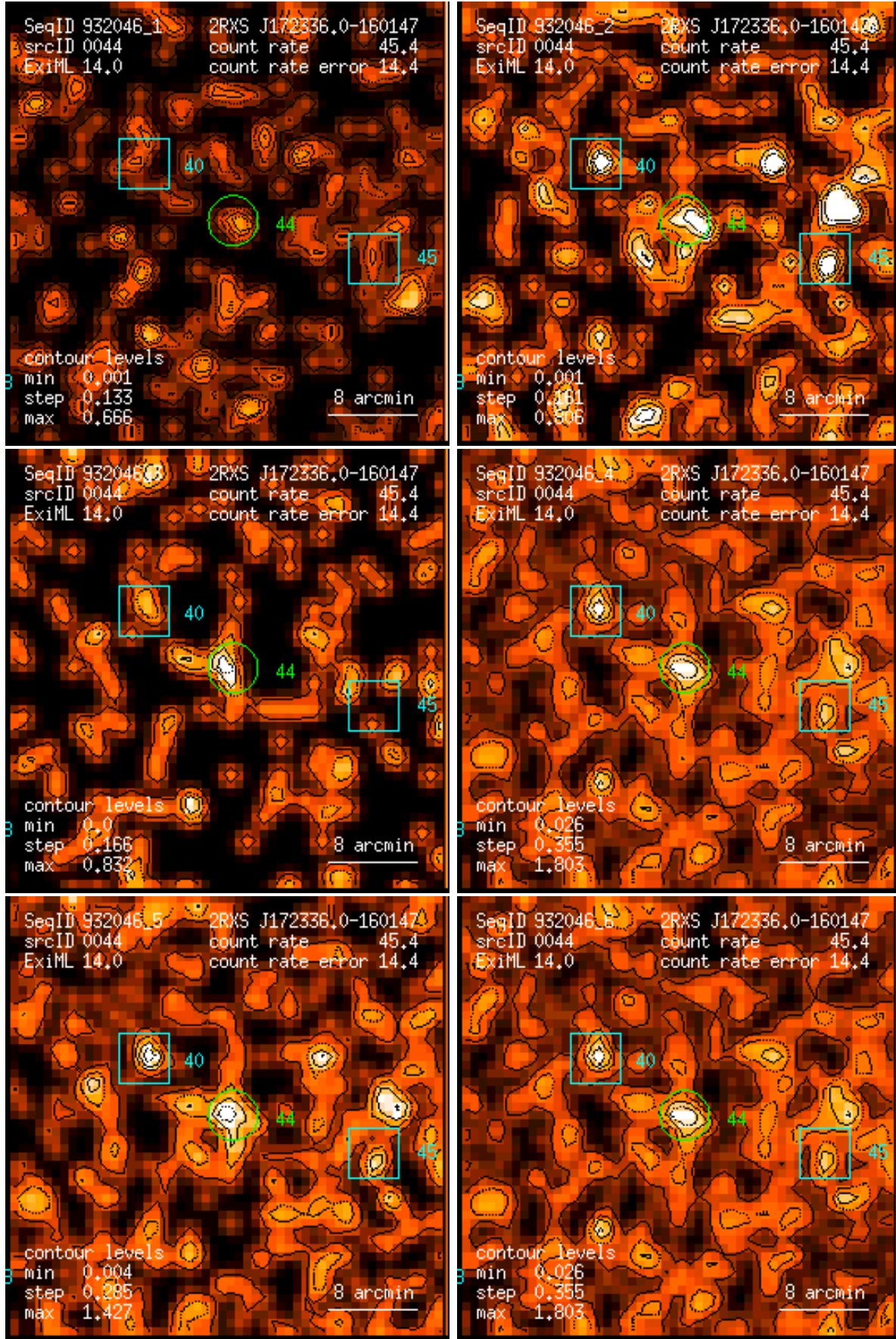
Figure 44: RASS 932046: detection 0044: band rate images, Gaussian filter: (1) PSPC channels 11 – 41, (2) 52 – 90, (3) 91 – 201, (4) 11 – 235, (5) 52 – 201, (6) 11 – 201. Broad band rates in counts/ks. Band rate contour levels in counts/ks/arcmin 2 .
