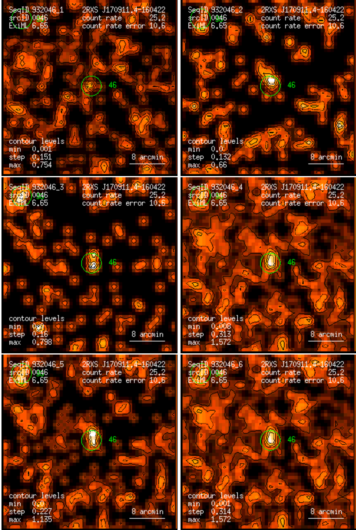
Figure 46: RASS 932046: detection 0046: band rate images, Gaussian filter: (1) PSPC channels 11 – 41, (2) 52 – 90, (3) 91 – 201, (4) 11 – 235, (5) 52 – 201, (6) 11 – 201. Broad band rates in counts/ks. Band rate contour levels in counts/ks/arcmin 2 .
