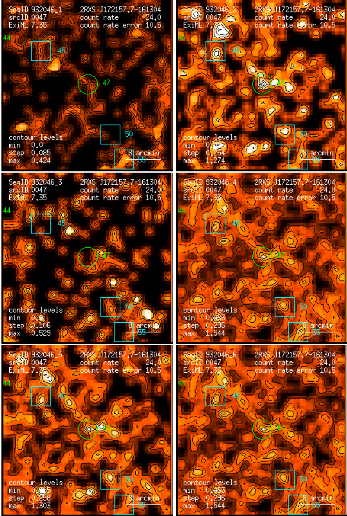
Figure 47: RASS 932046: detection 0047: band rate images, Gaussian filter: (1) PSPC channels 11 – 41, (2) 52 – 90, (3) 91 – 201, (4) 11 – 235, (5) 52 – 201, (6) 11 – 201. Broad band rates in counts/ks. Band rate contour levels in counts/ks/arcmin 2 .
