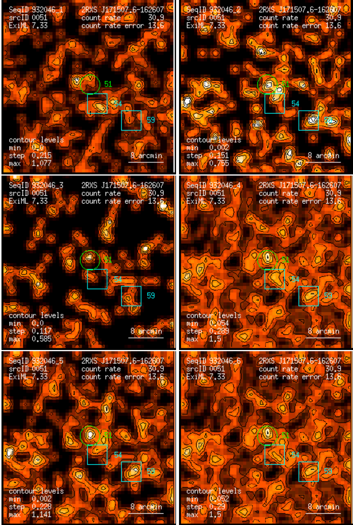
Figure 51: RASS 932046: detection 0051: band rate images, Gaussian filter: (1) PSPC channels 11 – 41, (2) 52 – 90, (3) 91 – 201, (4) 11 – 235, (5) 52 – 201, (6) 11 – 201. Broad band rates in counts/ks. Band rate contour levels in counts/ks/arcmin 2 .
