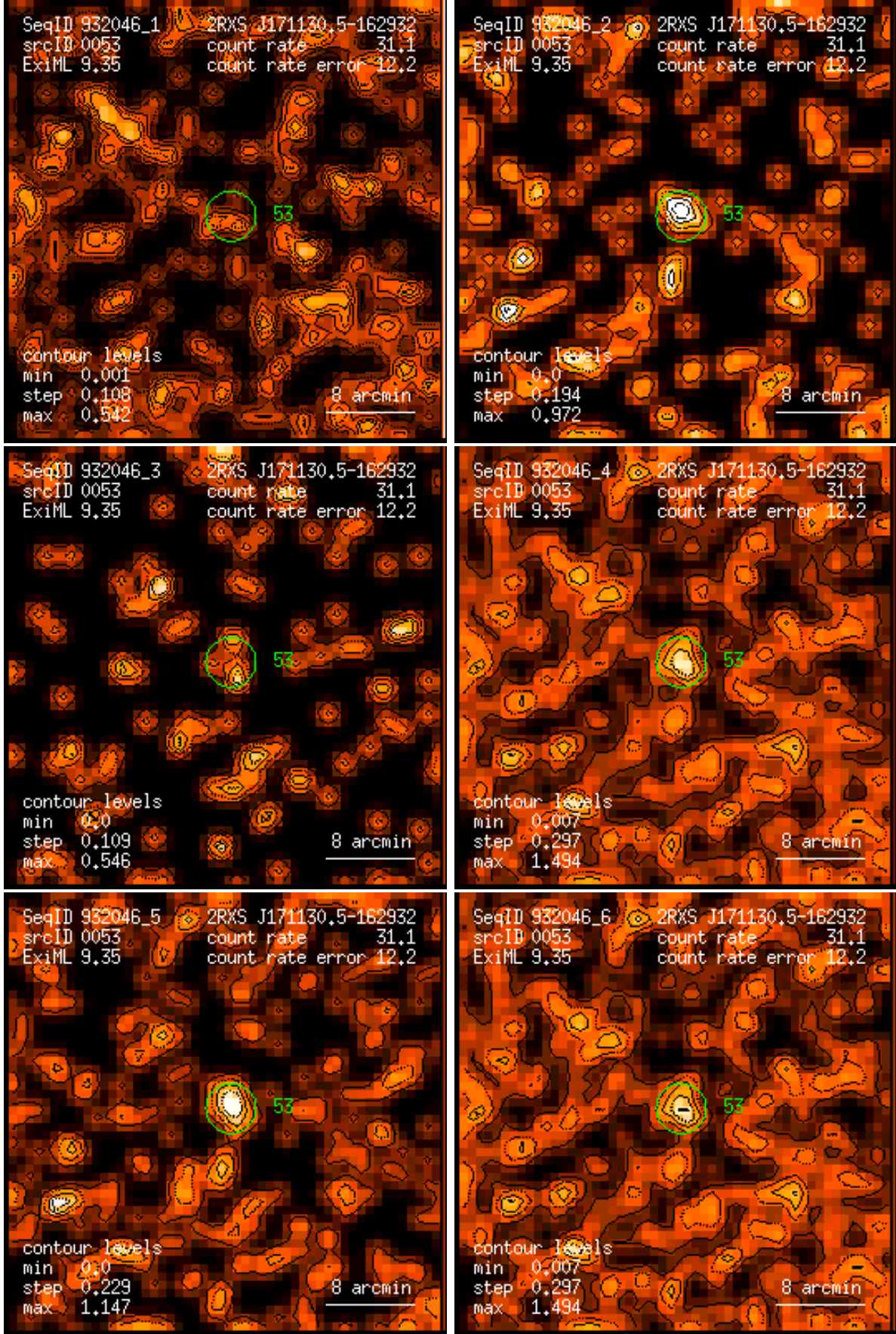
Figure 53: RASS 932046: detection 0053: band rate images, Gaussian filter: (1) PSPC channels 11 – 41, (2) 52 – 90, (3) 91 – 201, (4) 11 – 235, (5) 52 – 201, (6) 11 – 201. Broad band rates in counts/ks. Band rate contour levels in counts/ks/arcmin 2 .
