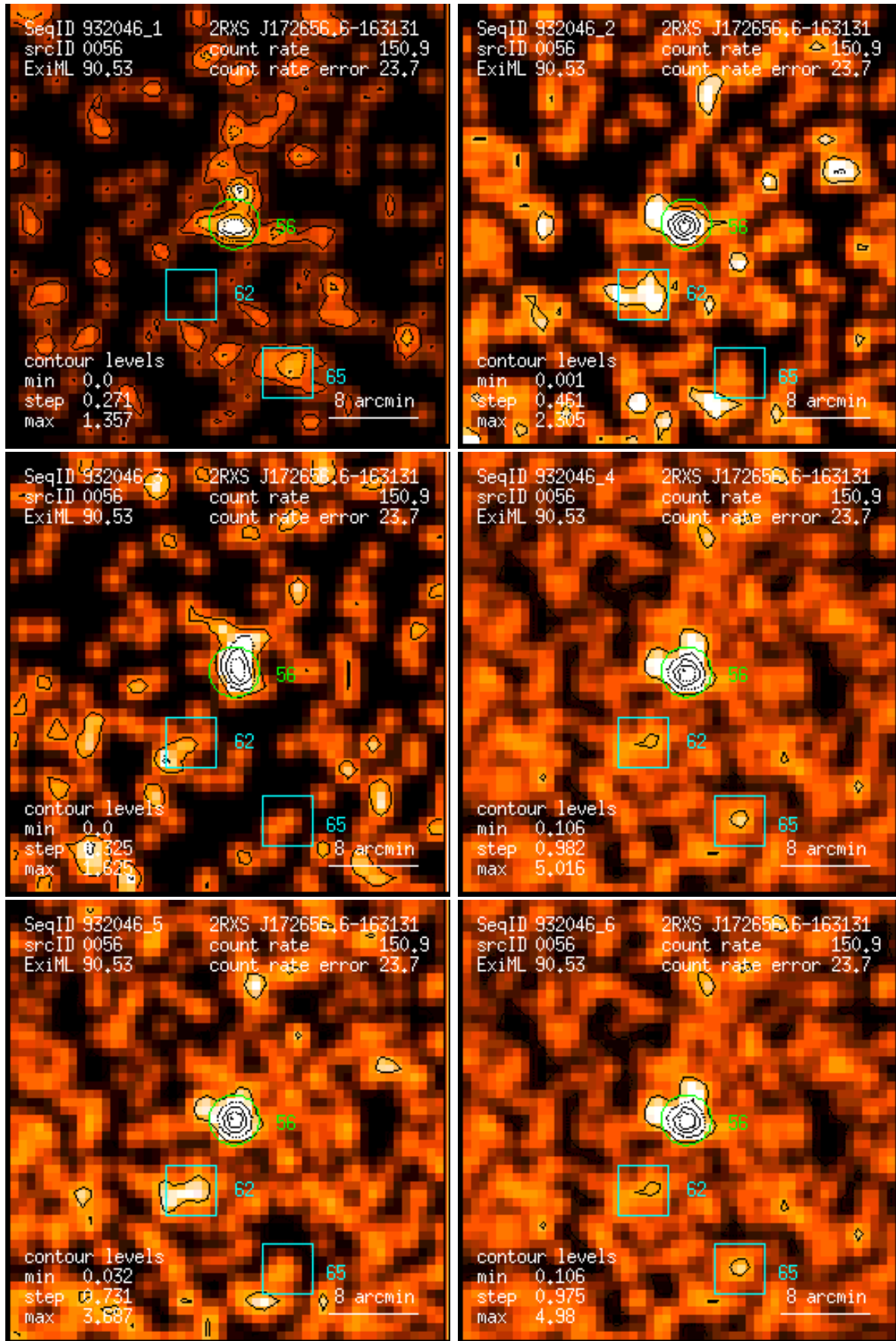
Figure 56: RASS 932046: detection 0056: band rate images, Gaussian filter: (1) PSPC channels 11 – 41, (2) 52 – 90, (3) 91 – 201, (4) 11 – 235, (5) 52 – 201, (6) 11 – 201. Broad band rates in counts/ks. Band rate contour levels in counts/ks/arcmin 2 .
