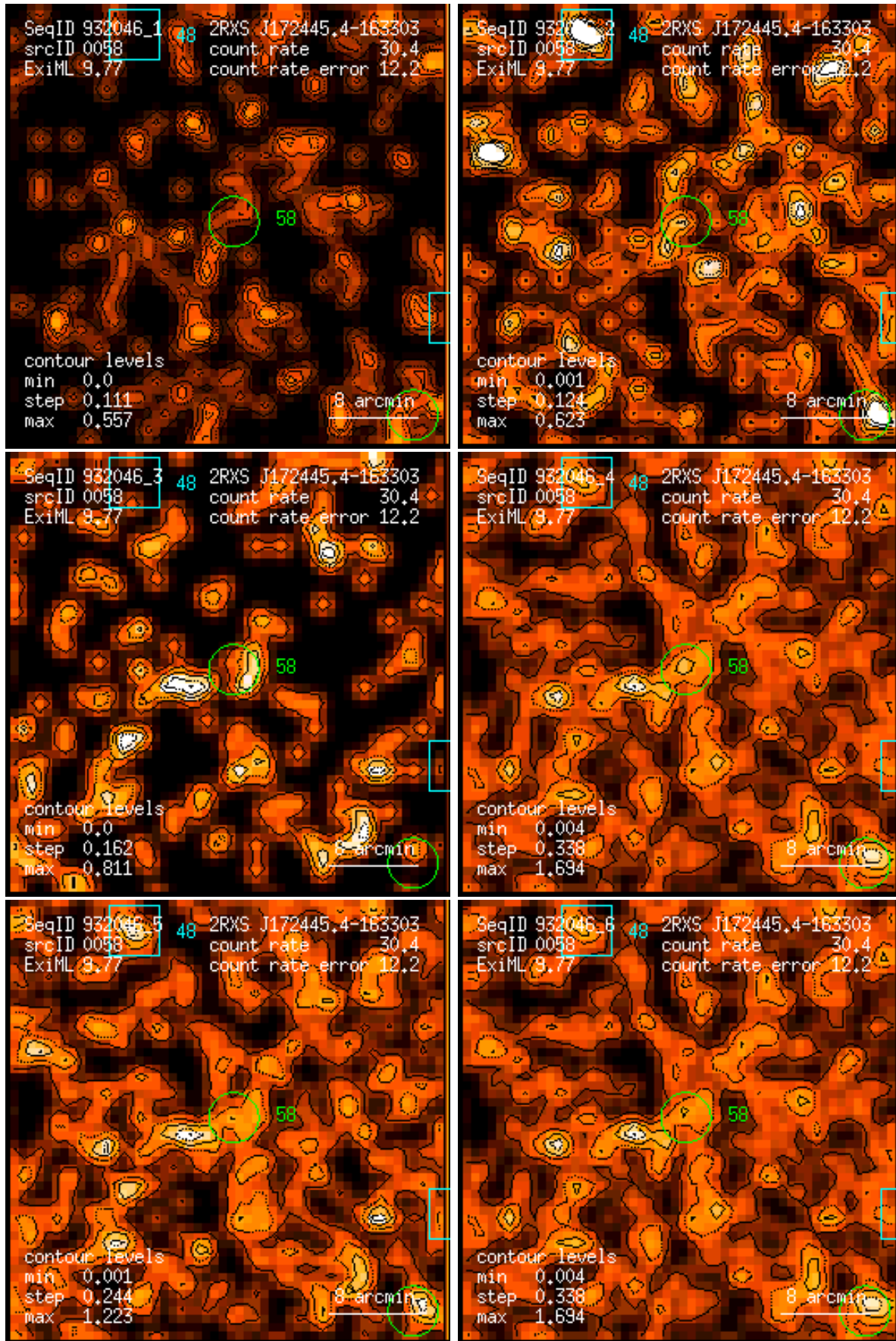
Figure 58: RASS 932046: detection 0058: band rate images, Gaussian filter: (1) PSPC channels 11 – 41, (2) 52 – 90, (3) 91 – 201, (4) 11 – 235, (5) 52 – 201, (6) 11 – 201. Broad band rates in counts/ks. Band rate contour levels in counts/ks/arcmin 2 .
