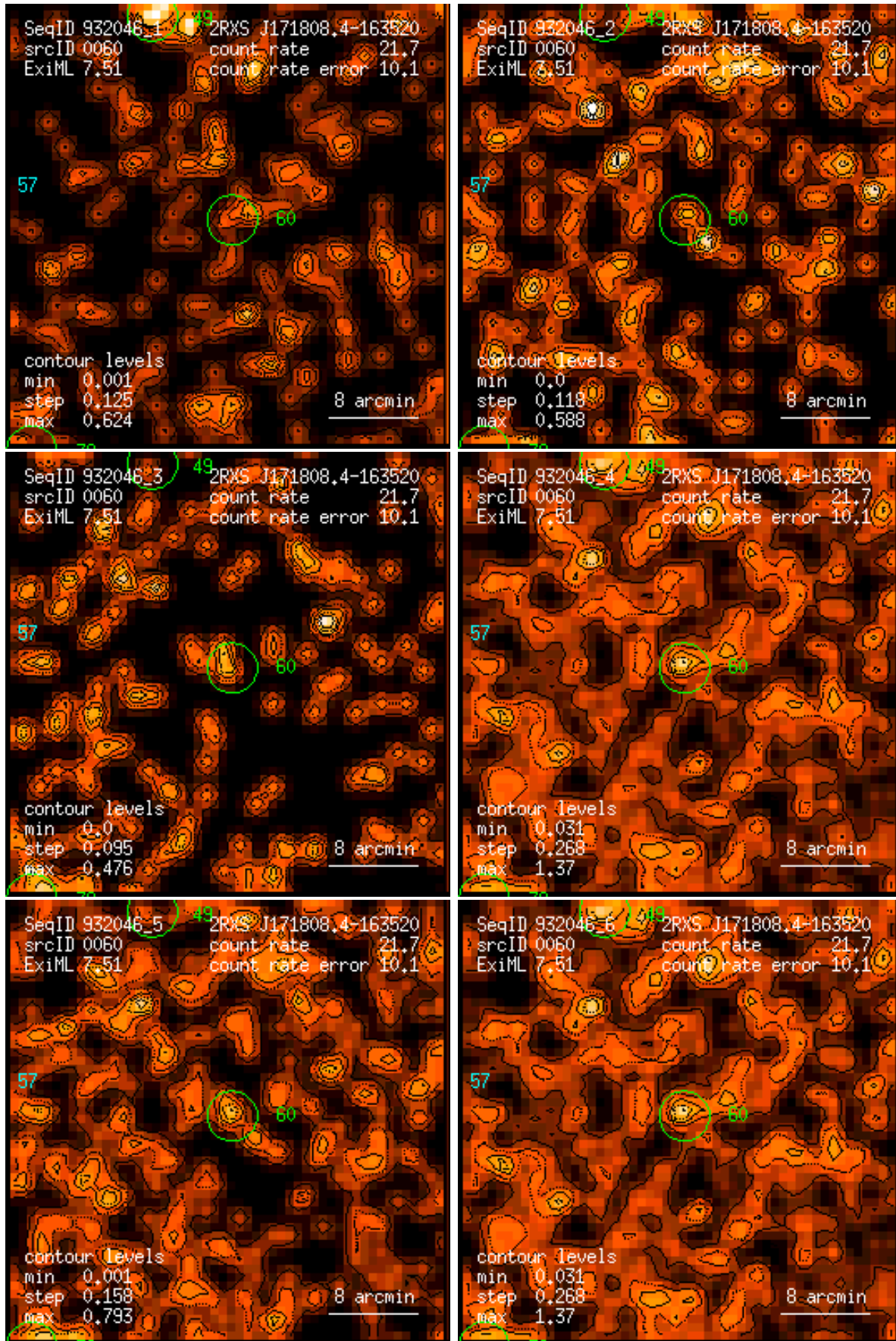
Figure 60: RASS 932046: detection 0060: band rate images, Gaussian filter: (1) PSPC channels 11 – 41, (2) 52 – 90, (3) 91 – 201, (4) 11 – 235, (5) 52 – 201, (6) 11 – 201. Broad band rates in counts/ks. Band rate contour levels in counts/ks/arcmin 2 .
