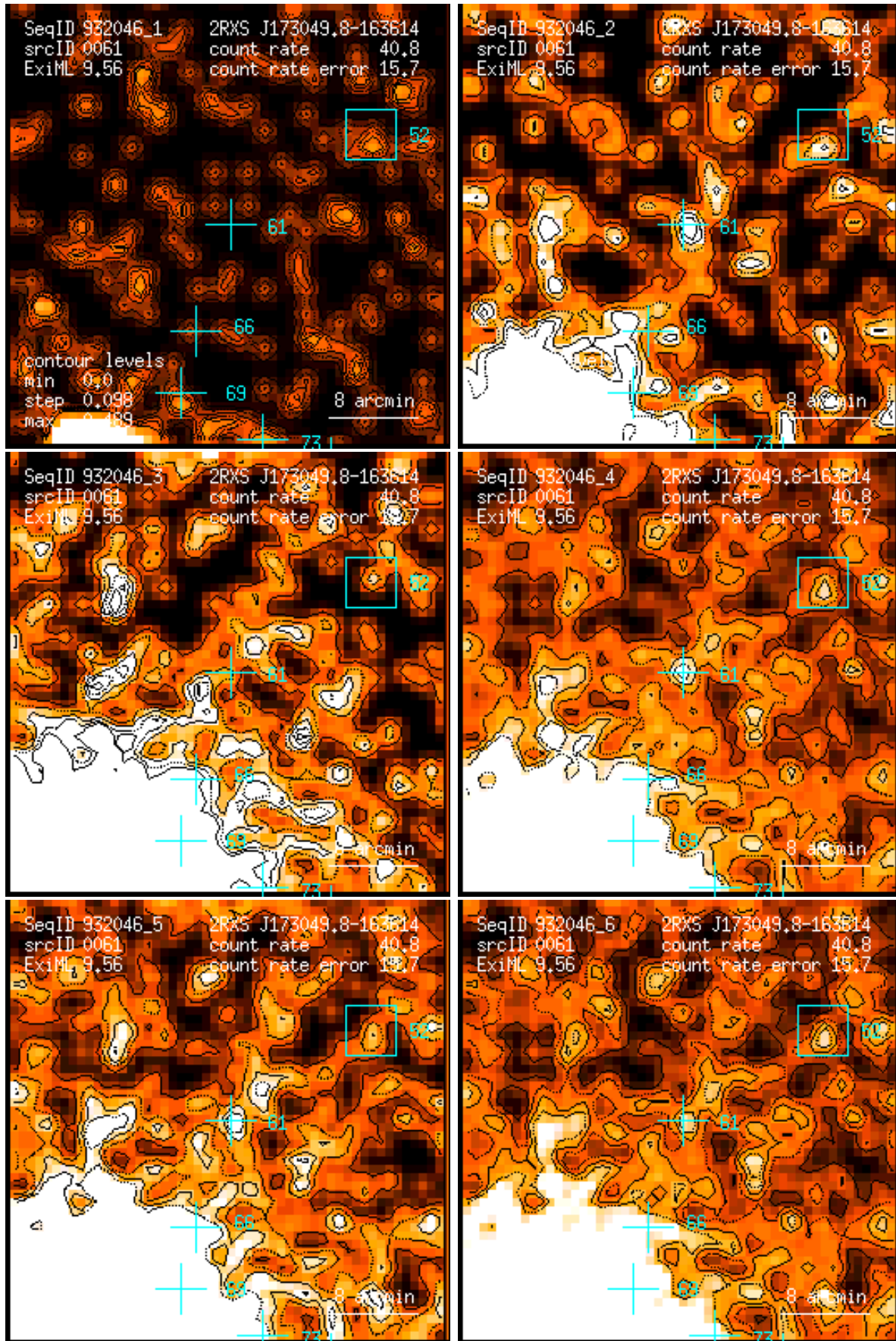
Figure 61: RASS 932046: detection 0061: band rate images, Gaussian filter: (1) PSPC channels 11 – 41, (2) 52 – 90, (3) 91 – 201, (4) 11 – 235, (5) 52 – 201, (6) 11 – 201. Broad band rates in counts/ks. Band rate contour levels in counts/ks/arcmin 2 .
