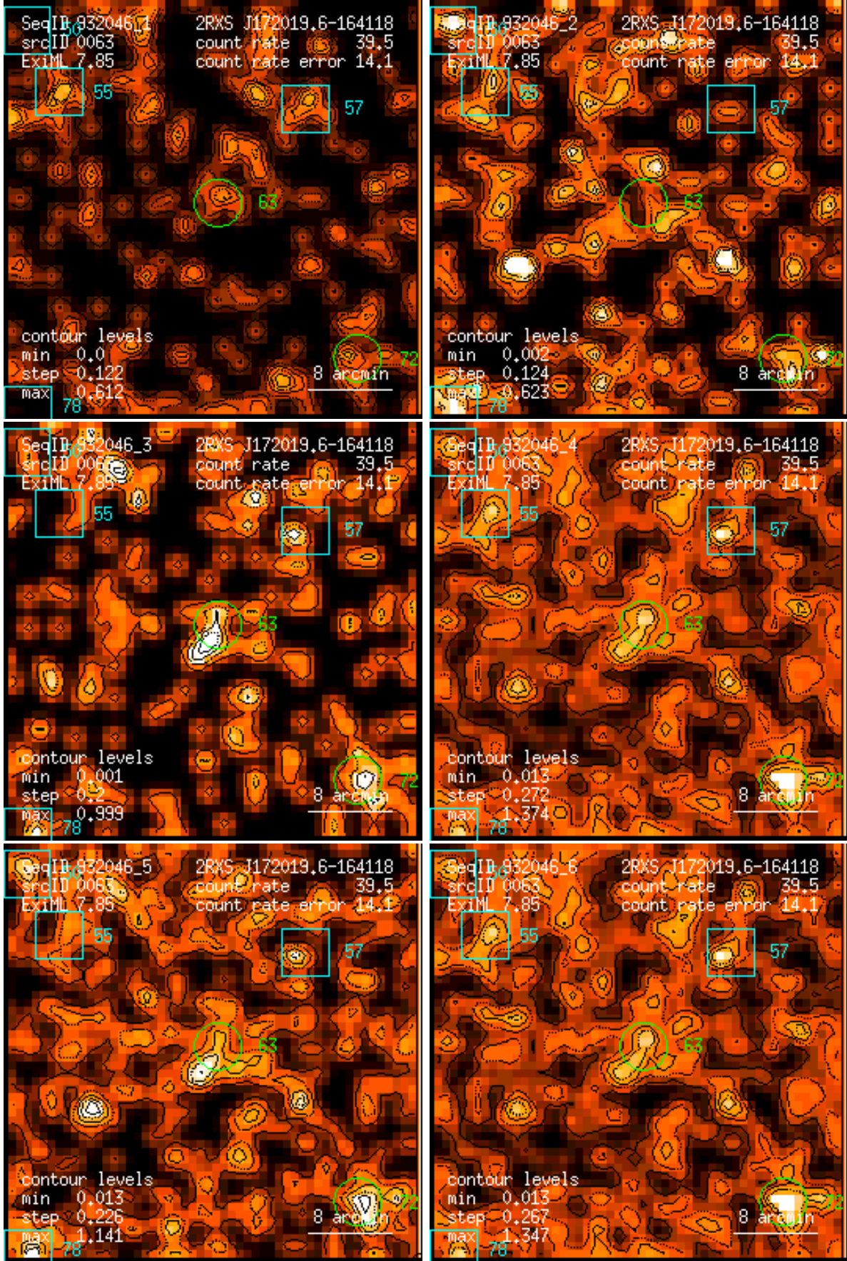
Figure 63: RASS 932046: detection 0063: band rate images, Gaussian filter: (1) PSPC channels 11 – 41, (2) 52 – 90, (3) 91 – 201, (4) 11 – 235, (5) 52 – 201, (6) 11 – 201. Broad band rates in counts/ks. Band rate contour levels in counts/ks/arcmin 2 .
